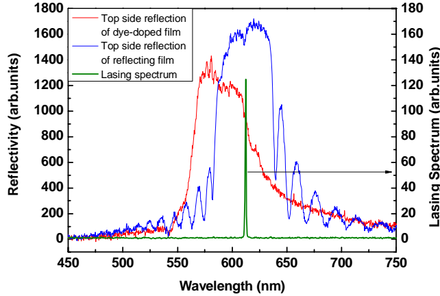
Fig. 2. Top side reflection bands of the 15 \mu\text{m} active film (red) and the 8 \mu\text{m} passive film (blue), and the lasing spectrum at 53 \mu\text{J}/\text{pulse} pump (green).
