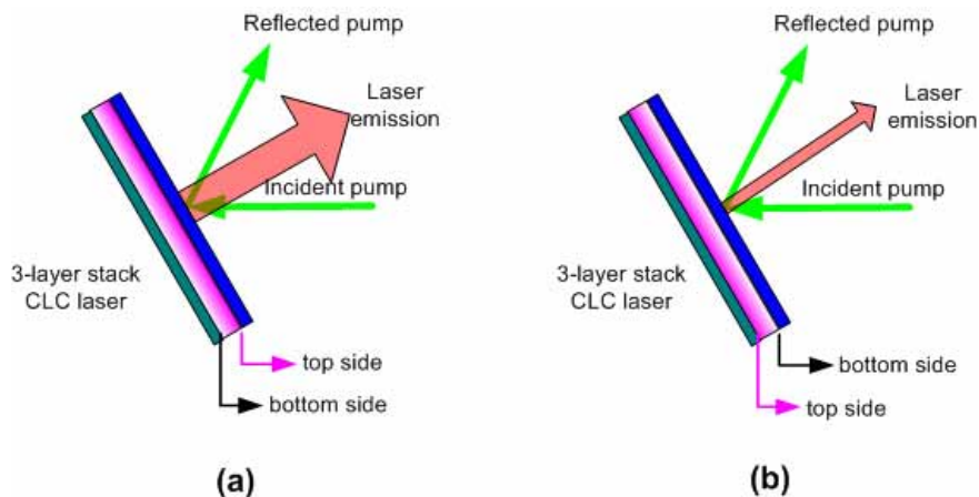
Fig. 4. Sample layout in the experimental setup: (a) top side of the active film is facing the pump beam and (b) bottom side of the active film is facing the pump beam. The 3-layer stack CLC laser: mirror (dark green) / active CLC film (magenta) / passive CLC film (blue).
