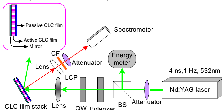
Fig. 1. Experimental setup: BS: Beam splitter; QW: Quarter-wave plate; CF: Color filter; LCP: left-handed circularly polarized light.
