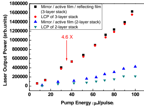
Fig. 3. The pump energy dependent laser output power of the total emission and LCP component from a {mirror/active CLC film/reflecting CLC film} laser and a {mirror/active CLC film} laser.
