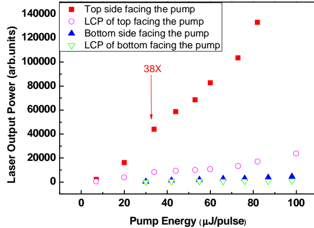
Fig. 5. The pump energy dependent laser output power from a single 15 \mu\text{m} active CLC film with the top side facing the pump source and the bottom side facing the pump source.
