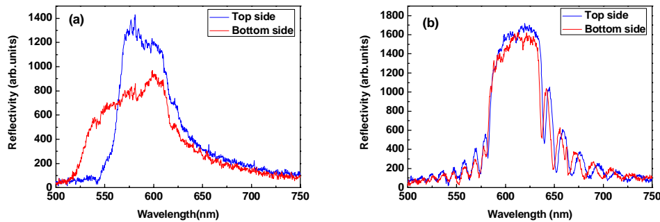
Fig. 6. The top side (blue) and bottom side (red) reflection bands of the CLC polymer film: (a) the 15 \mu\text{m} dye-doped CLC polymer film (b) the 8 \mu\text{m} passive CLC polymer film.
