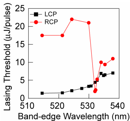
Fig. 3. Band-edge wavelength dependence of lasing threshold for the LCP and RCP pump beams. The band edge wavelength is controlled by the temperature.
