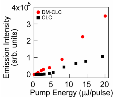
Fig. 6. Emission intensity as a function of pump energy of CLC with and without dielectric mirrors upon band-edge excitation.
