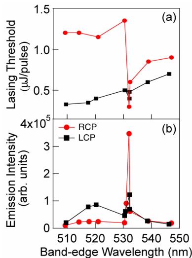
Fig. 5. (a). Lasing threshold and (b). emission intensity at 20 \mu\text{J}/\text{pulse} as a function of CLC band-edge wavelength.
