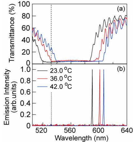
Fig. 2. Transmission and emission spectra of CLC as a function of temperature.
