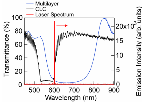
Fig. 4. Transmission spectra of the CLC cell, dielectric mirror, and laser spectrum of DM-CLC cell.
