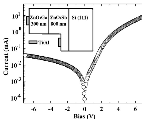
FIG. 1. Dark I - V curve of a ZnO:Ga/ZnO:Sb homojunction. Absolute value of current is plotted. Inset: Cross-sectional view of the diode. Shaded rectangles represent Ti/Al contacts.
