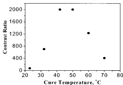
FIG. 2. The curing temperature dependent contrast ratio of the E48 LC gels containing 4% monomer concentration. Cell gap d = 8 \mu\text{m} , \lambda = 633 \text{ nm} , and T = 23 \text{ }^\circ\text{C} .
