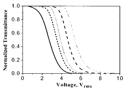
FIG. 5. The voltage-dependent transmittance of E48 LC gels with 2, 3, 4, 5, and 6 wt % (from left to right) monomer concentrations. The first-stage sample curing temperature is 50 °C. LC cell gap d=8\ \mu\text{m} , operating temperature T=23\ \text{°C} , and \lambda=633\ \text{nm} .
