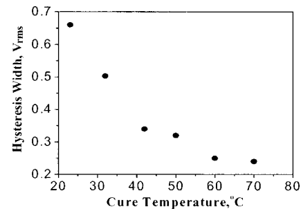
FIG. 3. The curing temperature dependent hysteresis of the E48 LC gels containing 4% monomer concentration. Cell gap d = 8 \mu\text{m} , \lambda = 633 \text{ nm} , and T = 23 \text{ }^\circ\text{C} .
