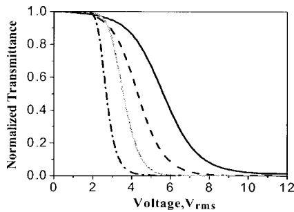
FIG. 1. The voltage-dependent transmittance of the E48 LC gels at 23, 32, 50, and 70 °C curing temperatures (from right to left). Cell gap d = 8 \mu\text{m} , monomer concentration 4 wt %, laser wavelength \lambda = 633 \text{ nm} , and measurement temperature T = 23 \text{ }^\circ\text{C} .
