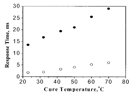
FIG. 4. The curing temperature dependent rise time (open circles) and decay time (close circles) of the 8 \mu\text{m} E48 LC gels with 4% monomer concentration. For each cell, the rise and decay times were measured between V = 0 and the corresponding dark state voltage shown in Fig. 1.
