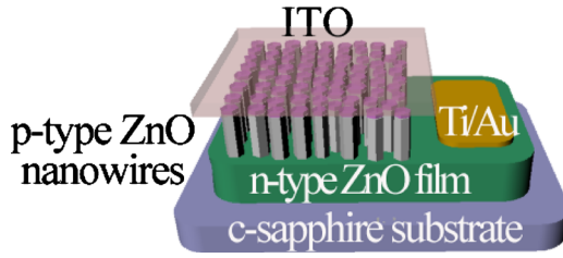
FIG. 1. (Color online) Schematic view of the photodetector device, which consists of ZnO thin film on c-sapphire substrate, vertically aligned ZnO nanowires, ITO contacts, and Ti/Au contacts.
