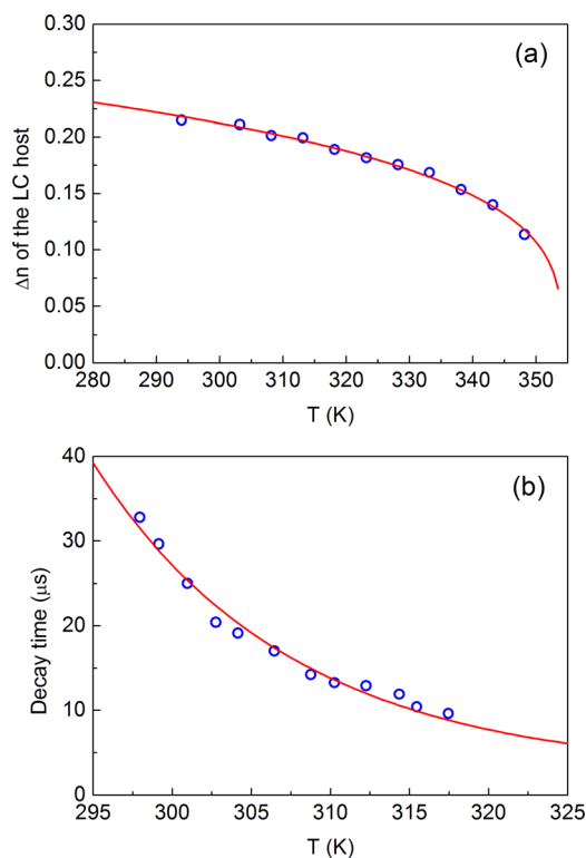
FIG. 3. (Color online) (a) Temperature dependent \Delta n of the LC host JM2069-145 and (b) temperature dependent decay time for the VFS PSBP cell. Blue dots: experimental data; Red line: fitting curve.
