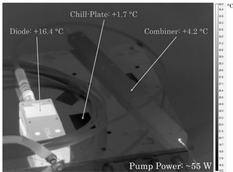
Figure 27. Thermal image of pump diode, water-chilled plate, and pump combiner at maximum pump power of ~55 W. Printed temperatures are relative to temperatures with no pump.
