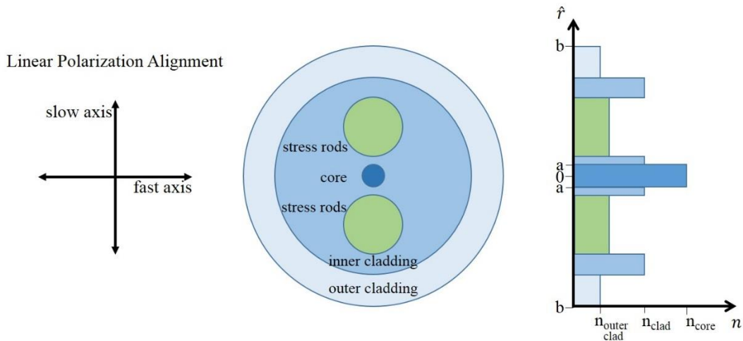
Figure 3. PM-DC-SIF. Left: Preferred input polarization to maintain linear output polarization. Right: Cross-sectional refractive index profile.
