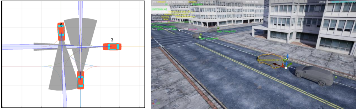
Figure 12: Simulation of the visual behavior of a driver through a field-of-view in early MATLAB prototype (left); and in the current iteration of the simulator (right)
