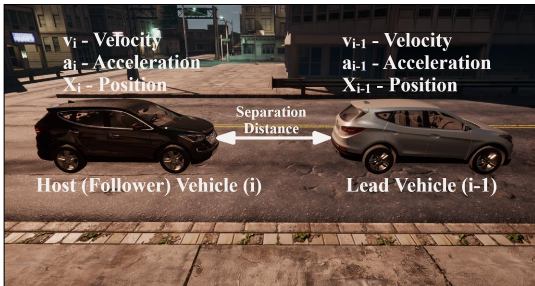
Figure 35: A scenario of two vehicles with variables of interest
