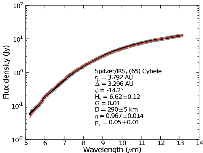
Fig. 1. Flux density spectrum of Cybele in the mid-infrared (points) and best-fit NEATM (red line).
