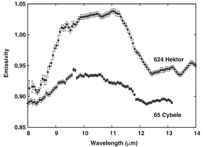
Fig. 5. Emissivity spectrum of Cybele compared to that of Trojan asteroid (624) Hektor (shifted in the emissivity axis for clarity). Notice the emission plateau due to fine silicate grains in the spectrum of both asteroids. Notice also that the contrast is smaller ( \sim 5\% ) in the spectrum of Cybele than in that of Hektor ( \sim 15\% ).
