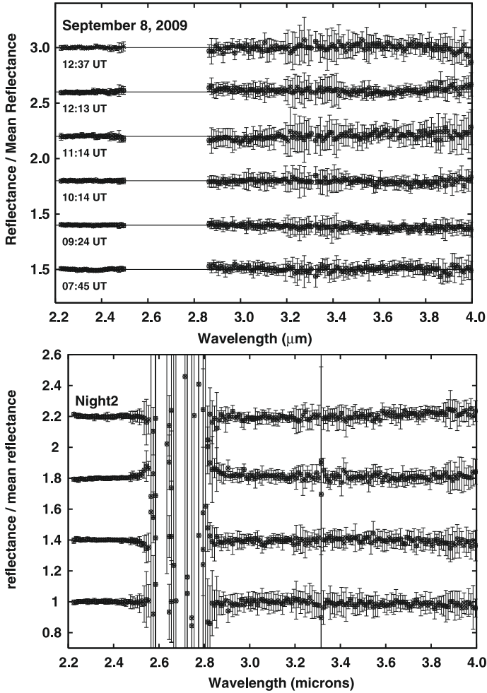
Fig. 3. IRTF spectra of Cybele divided by the mean spectrum of each night, shifted in reflectance for clarity. Notice that no significant differences are shown within the S/N .
