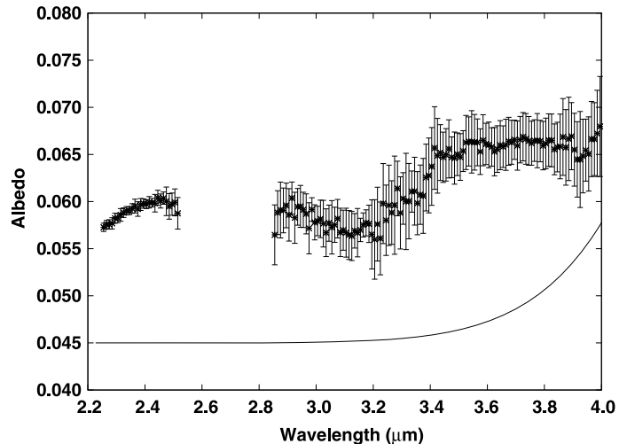
Fig. 6. Mean spectrum of Cybele in the 2–4 \mu\text{m} range. The thermal contribution was subtracted and the reflectance transformed to albedo units (see text). The thermal contribution is shown as a solid line (scaled to albedo units and shifted by 0.045 to fit in the figure). Notice that the thermal contribution in the 3.1 \mu\text{m} band is negligible.
