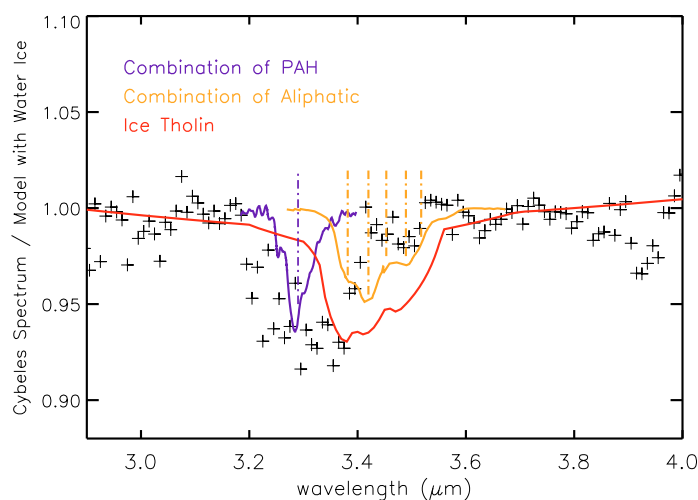
Fig. 8. The residuals of dividing Cybele’s spectrum against the model are shown (as crosses) together with the spectra of organics with different composition. In yellow is the spectrum of a sample of Insoluble Organic Material from Orthous-Dauna et al. (2010) showing the contribution of the aliphatic structure. The purple line is the spectrum of an average of six polycyclic aromatic hydrocarbons from Colangeli et al. (1992). The red line is the spectrum of ice tholin from Khare et al. (1993).
