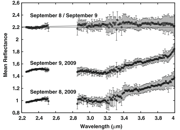
Fig. 4. Mean spectrum of Cybele obtained on September 8 and 9, shifted in reflectance for clarity, and the division of both (also shifted). Notice that the differences are only significant in the slope, the September 9 spectrum being slightly redder by about 0.5\%/0.1 \mu\text{m} .
