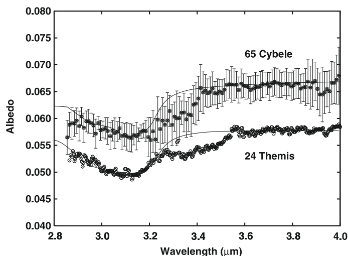
Fig. 7. Reflectance spectrum of Cybele and Themis in albedo units. Within the noise, both spectra looks very similar. Overplotted on the spectrum of Themis is the spectral model included in Fig. 1 of Rivkin & Emery (2010). A similar model is overplotted on Cybele’s spectrum. These models include a thin coating of H 2 O ice on surface grains. Notice that models fit very well the left part of the band while at longer wavelengths there are additional absorptions.
