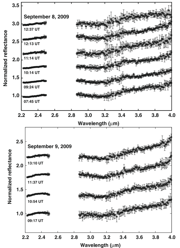
Fig. 2. IRTF reflectance spectra of Cybele normalized at 2.4 \mu\text{m} , obtained in both nights and shifted in reflectance for clarity.
