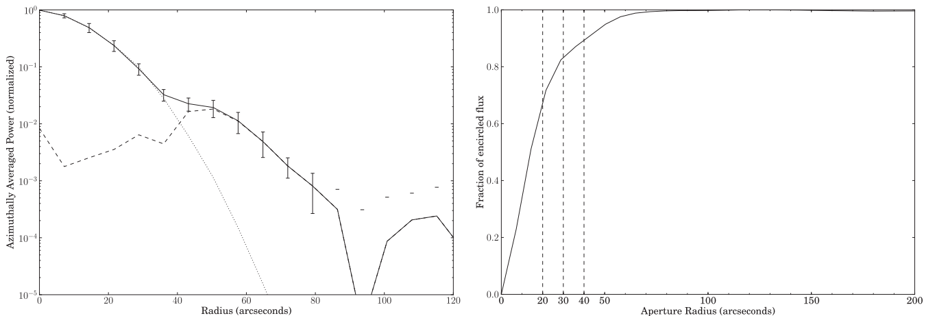
Figure 14. Left: the radial profile (solid) of the Bolocam PSF derived from Neptune and Uranus observations, including all bolometers. The main lobe is well approximated by a Gaussian (dotted) and the sidelobes are due to the Airy pattern from truncation of the beam at the cold Lyot stop (dashed). Error bars indicate the azimuthal standard deviation. Right: enclosed flux in an aperture of a given radius based on the measured PSF. This curve is the basis of the point source aperture corrections (Table 2). Vertical dashed lines indicated 20, 30, and 40 arcsec radii.
