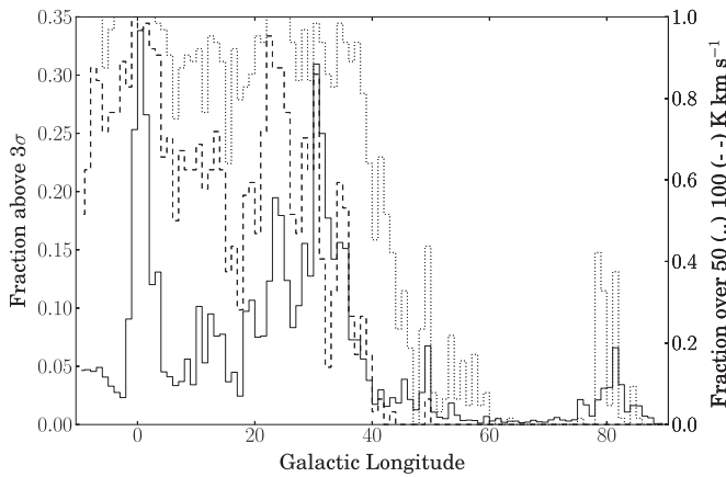
Figure 23. Filling factor of millimeter continuum emission from the BGPS compared to CO(1 → 0) emission from Jackson et al. (2006). The axis on the left side gives the filling fraction above 3\sigma of the local rms from the BGPS (solid line). The right axis gives the CO filling fraction above 50 (dotted) and 100 (dashed) K km s -1 .
