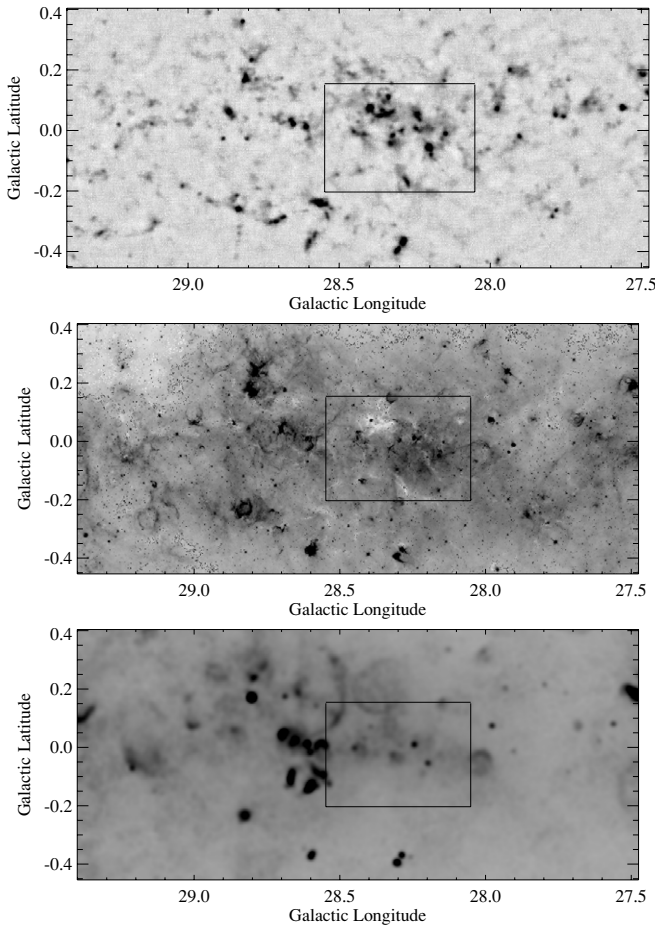
Figure 20. View of 2 \text{ deg}^2 of the Galactic Plane centered at l = 28.45 , b = 0 . Top: BGPS, middle: Spitzer -GLIMPSE 8 \mu\text{m} ( 1''.9 ), and bottom: VGPS 20 cm continuum ( 40'' ). IRDCs appear in the Spitzer negative image as wispy white regions against the gray emission background. While some of the Bolocam sources are apparent as IRDCs or strong infrared or radio sources, many lack any apparent association with features at these wavelengths. The box indicates the zoom-in region in Figures 21 and 22.
