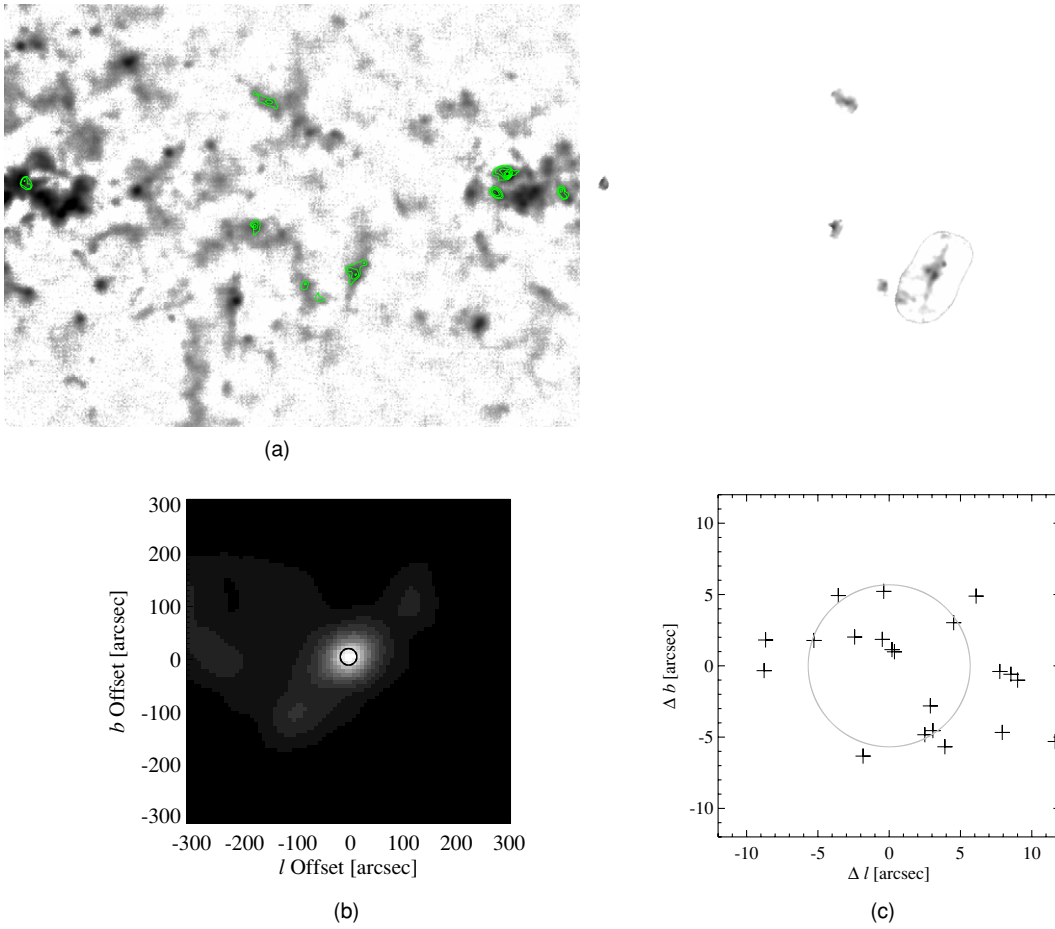
Figure 5. Comparing the Bolocam positions to those of the SCUBA Legacy Catalog. (a) Left: the Bolocam map in a portion of the l = 30 field. Right: the SLC maps in the same region. The green contours on the Bolocam map indicate the positions of the SLC sources. Note that the SLC maps only cover a small portion the entire region shown, corresponding to the isolated sources indicated by the contours. Negative bowls in both images are forced to zero before cross-correlating. (b) The cross-correlation map of the BGPS and SLC maps in (a). (c) The measured offset between Bolocam and SCUBA Legacy sources (Di Francesco et al. 2008), using the method described in Section 3.4. The circle indicates the 1\sigma region, which is also consistent with the error derived from the internal Bolocam pointing model.
