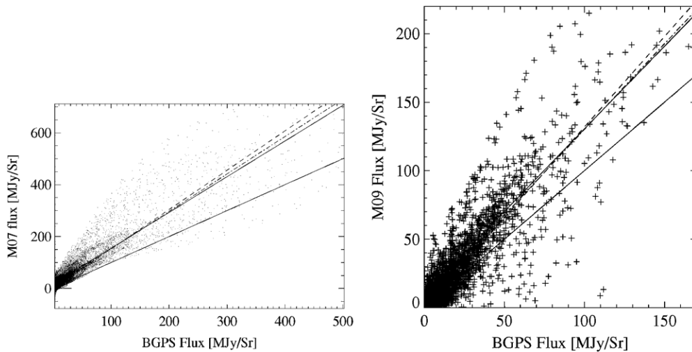
Figure 17. Left: a plot of the values of the pixels in the M07 and BGPS maps after both have been convolved to the same resolution on the same grid. The solid line is the expected 1:1 correspondence; the other lines show the slopes obtained with various lower bounds as given in Table 3. There is clearly a great of scatter about the mean. Right: the same analysis, but for the M09 SIMBA data.
