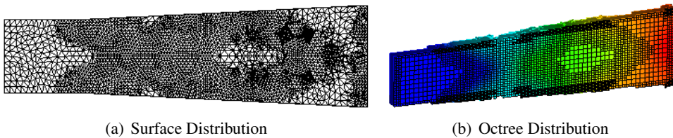
Figure 6: Point Distributions for Supersonic Expanding Nozzle
