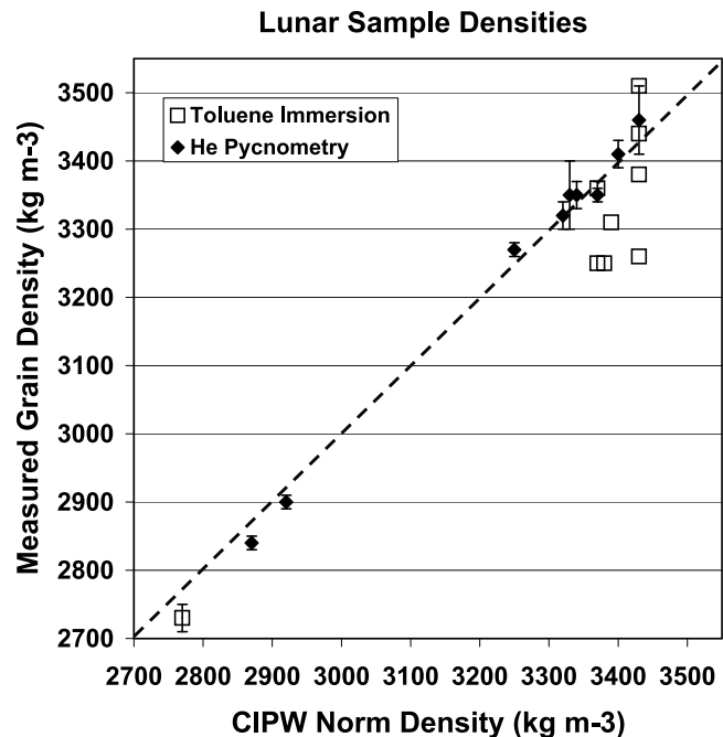
Figure 1. Measured grain density versus the normative mineralogy density for basalts and gabbros measured by helium pycnometry (filled diamonds) and by toluene immersion (open squares). Normative mineralogy densities are from Table S2. Grain densities by He pycnometry are from Table 1. Grain densities by toluene immersion are from Fujii and Osako [1973], Horai and Winkler [1975, 1976, 1980], Ahrens et al. [1977], Jeanloz and Ahrens [1978], and Ahrens and Watt [1980]. The dashed line represents perfect agreement between the measured and theoretical densities.
