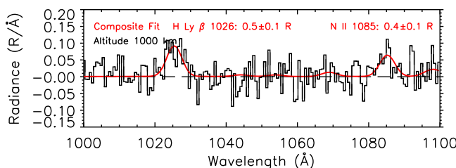
Figure 2. UVIS Titan EUV airglow data while in Saturn’s shadow. The composite fit to the data is overplotted in red and the altitudes over which the data is averaged are the same as in Figure 1. The H Ly \beta and N II 1085 \text{ \AA} radiance is indicated with the fitted uncertainty.
