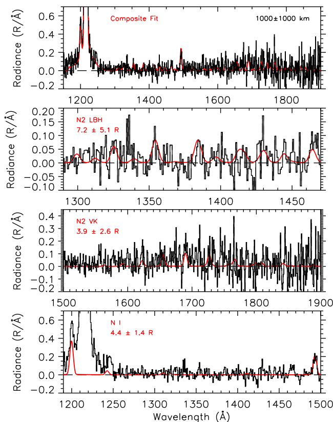
Figure 1. (top) UVIS Titan FUV airglow data on 7 May 2009 between 8:27 and 10:50 UT while in Saturn’s shadow. The composite fit to the data is overplotted in red and the altitudes over which the data is averaged are indicated. (top middle) Same as Figure 1 (top) but showing the component of the fit from the N_2 LBH bands Radiances and uncertainties from the fit over the wavelength region in Figure 1 (top) are indicated. (bottom middle) Same as Figure 1 (top middle) but showing the component of the fit from the N_2 VK bands instead. (bottom) Same as Figure 1 (top middle) but only showing the component of the fit from the N I features.
