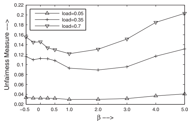
Fig. 9 Unfairness measure versus \beta under c_1 .
