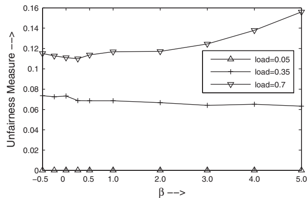
Fig. 10 Unfairness measure versus \beta under c_5 .
