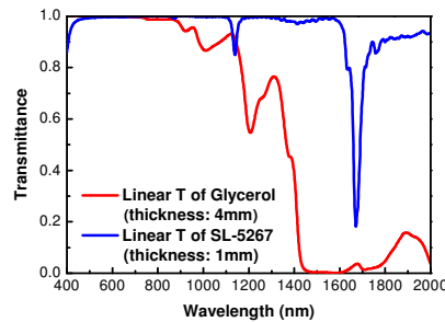
Fig. 3. Transmission spectra of SL-5267 and Glycerol measured from 400 nm to 2000 nm.
