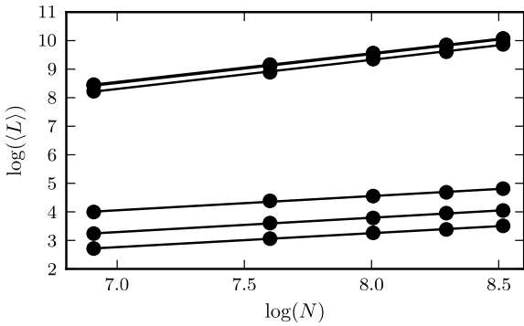
Fig. 4. Scaling of the average length \langle L \rangle as a function of lattice sites N . \log(\langle L \rangle) was fitted to \beta \log(N) + b . The \gamma = -1 and “tanh” action coincide at the top line, the second line is for the “sin” action, the third for \gamma = 0.5 , the fourth for \gamma = 1.0 and the fifth for \gamma = 2.0 .
