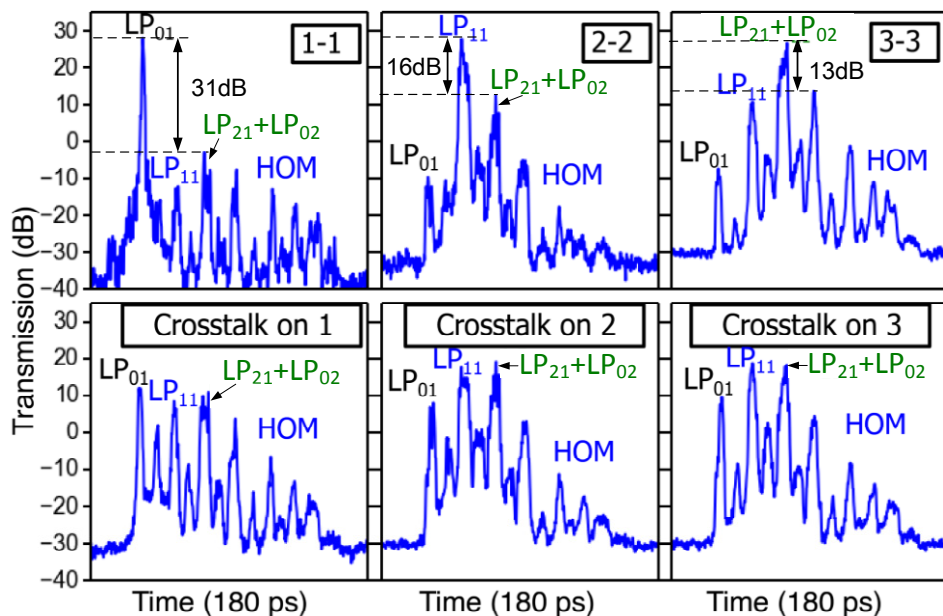
Fig. 9. Summation of signal and crosstalk cells from reflection transfer matrix for mode group selective lantern supporting three mode groups.
