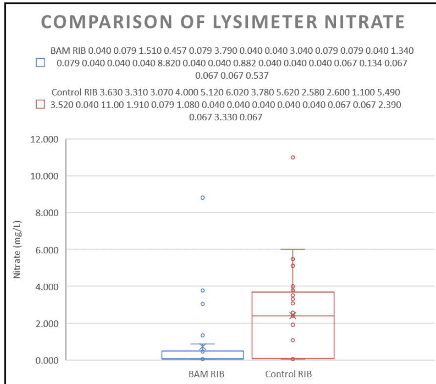
Legend: Reference EXCEL 2016: average x, minimum ⊥, maximum ⊤, Quartiles — Figure 13 Comparison of Nitrate under the BAM and Control RIBs Using Reclaimed Water
