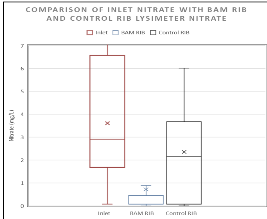
Legend: Reference EXCEL 2016: average x, minimum \perp , maximum \top , Quartiles \text{—|—} Figure 14 Comparison of Inlet and Lysimeter Nitrate Concentrations Using Reclaimed Water
