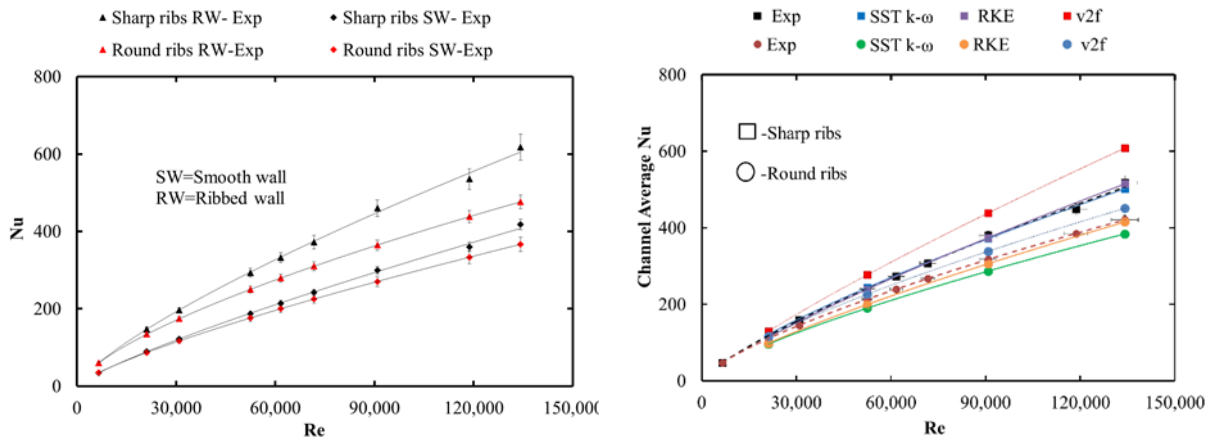
a) Smooth and ribbed wall Nu vs. Re
