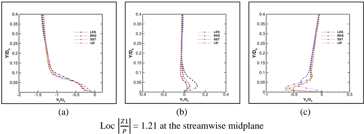
Figure 32 Comparative mean velocity results between LES and different RANS models at Re \approx 30k
