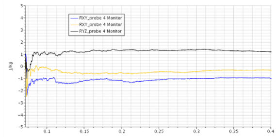
Figure 87 Statistical convergence of LES
