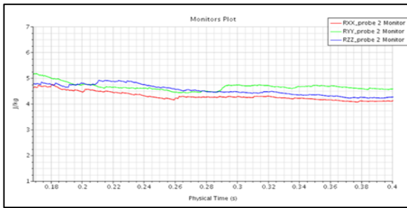
Figure 21 Statistical convergence of LES
