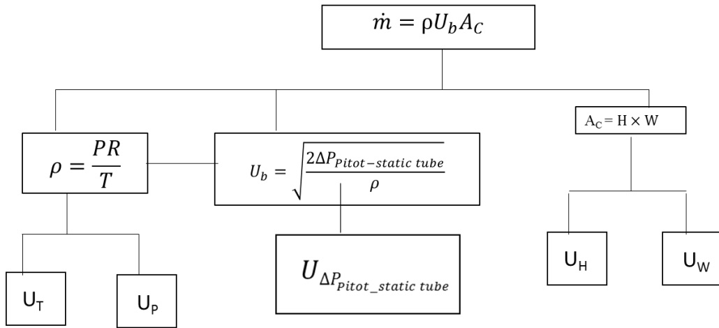
Figure 76 Uncertainty tree for mass flow rate
