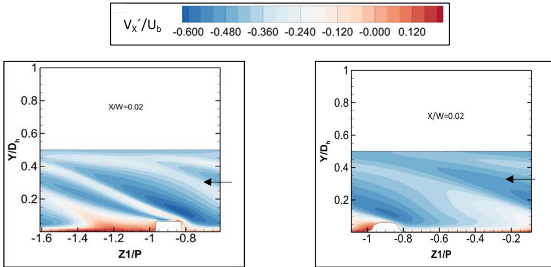
Figure 69 Non-dimensional V_x' contour plot at the streamwise plane at X/W = 0.02
