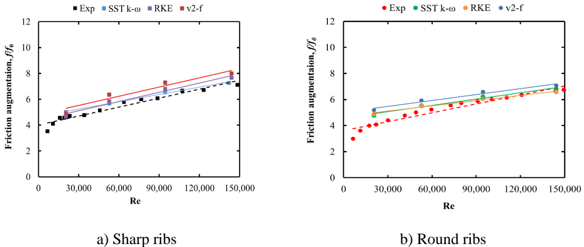
Figure 26 CFD results of friction augmentation at different Re
