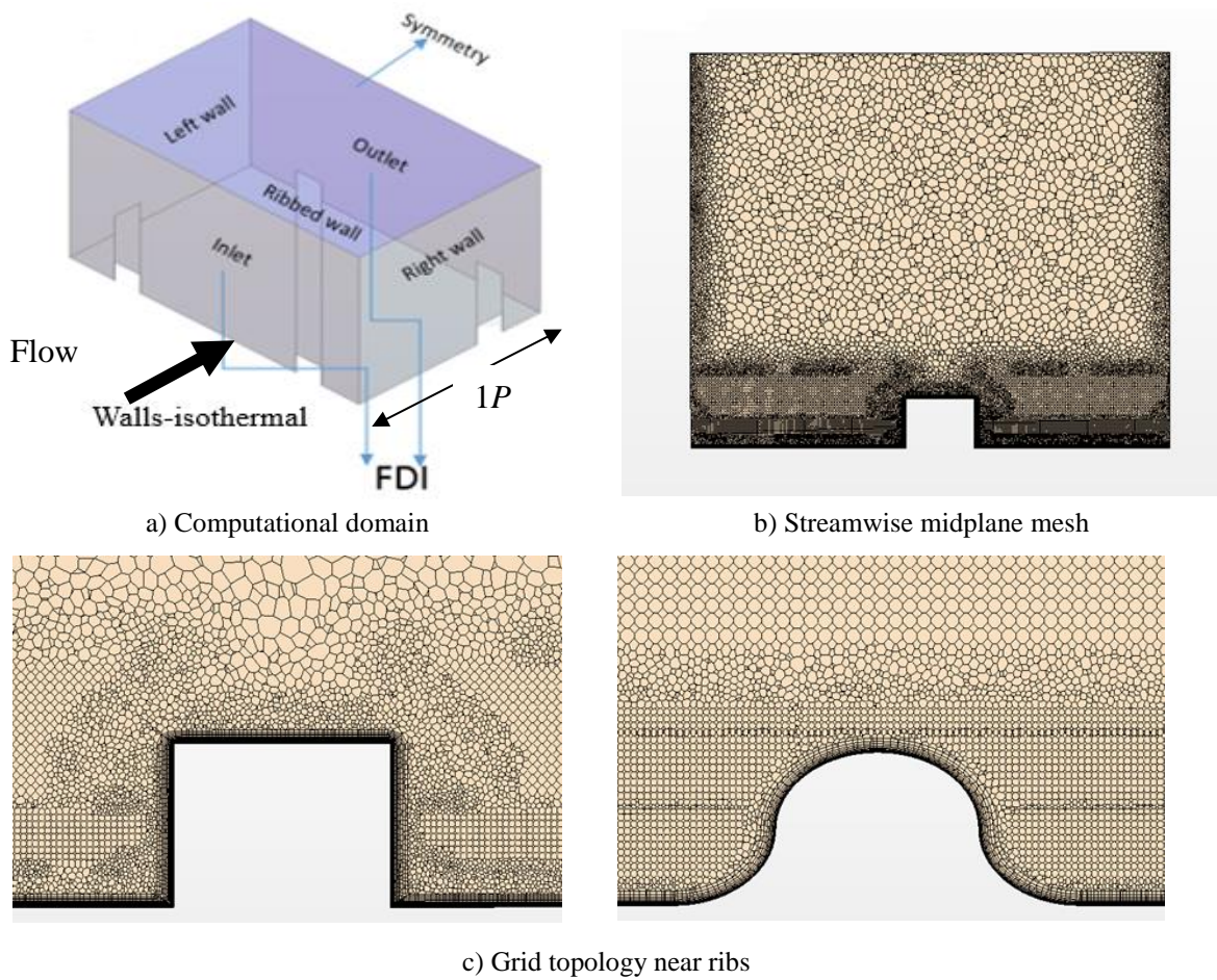
Figure 16 Computational domain and grid topology for two ribbed wall cases
