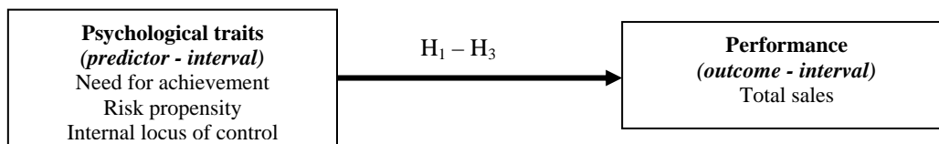
Figure 1: Theoretical Framework
