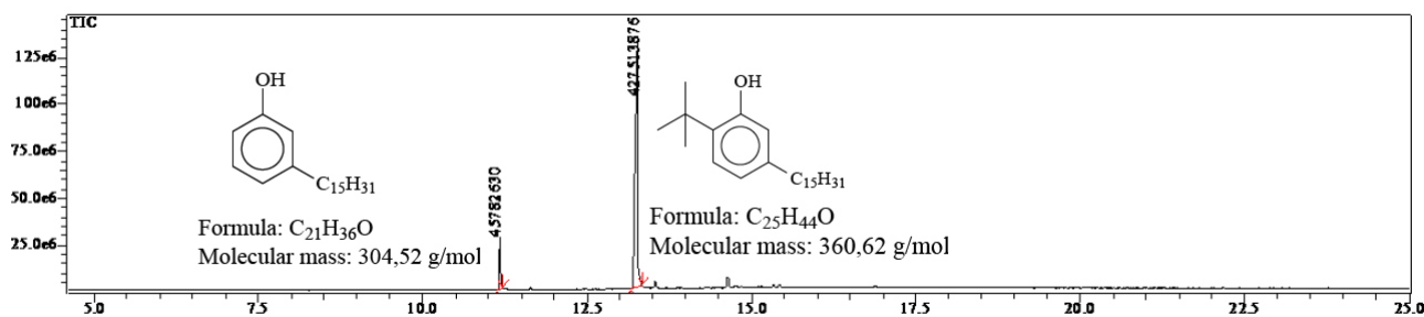
Figure 1 Chromatogram of Blend (A2)
