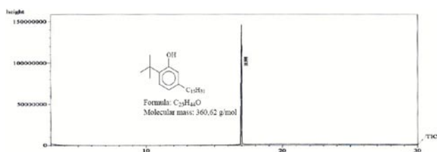
Figure 2 Chromatogram of 5- n -pentadecyl-2- tert -butylphenol (A3)
