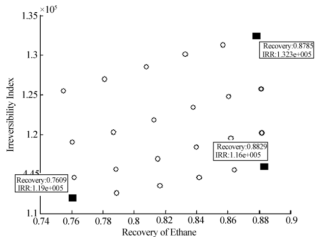
Figure 9 Irreversibility Index vs. Recovery in 24 Different Position of Pump-Around
