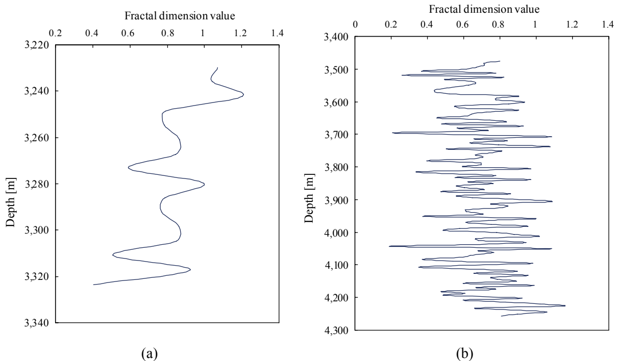
Figure 2 Distribution of Vertical Fractal Dimension Value. (a) Su53-4, (b) Su 53-78-46H
