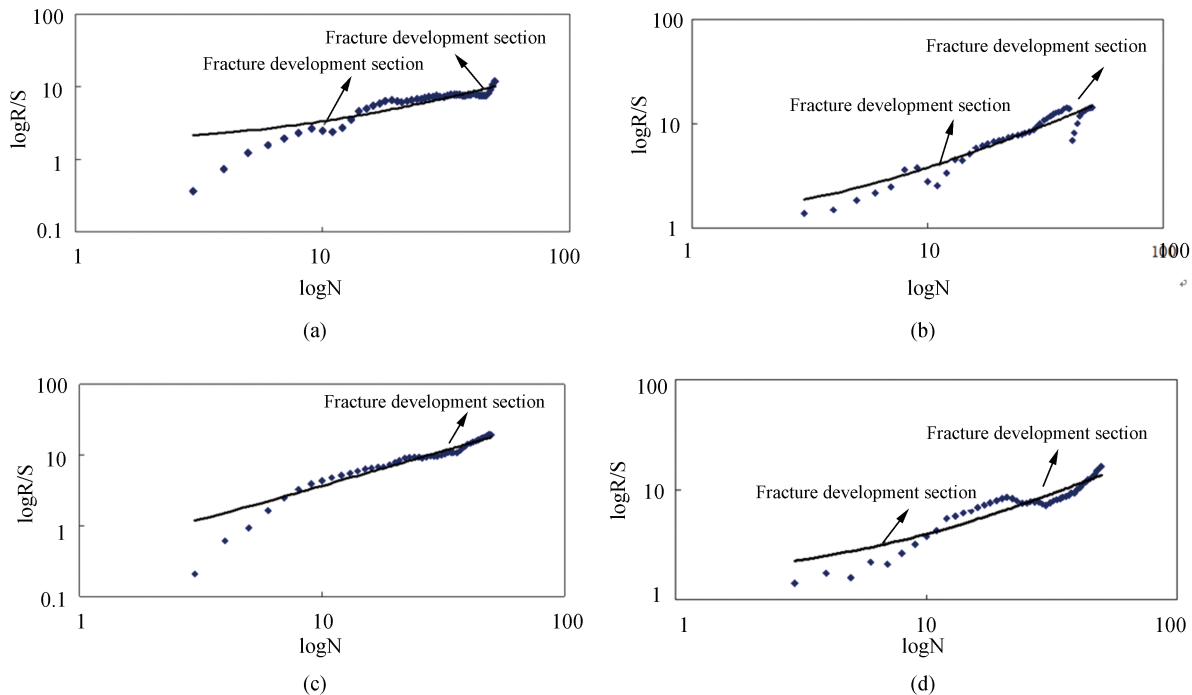
Figure 1 The Double Logarithmic Relationship Diagram Between R/S and n of the Amplitude Difference Data. (a) Su53-4, Depth Interval: 3,229.735 - 3,235.860 m, (b) Su53-8, Depth Interval: 3,168.25 - 3,174.375 m, (c) Su 53-78-46H, Depth Interval: 3,475.625 - 3,481.75 m, (d) Su 53-78-58H, Depth Interval: 3,395.825 - 3,401.95 m
