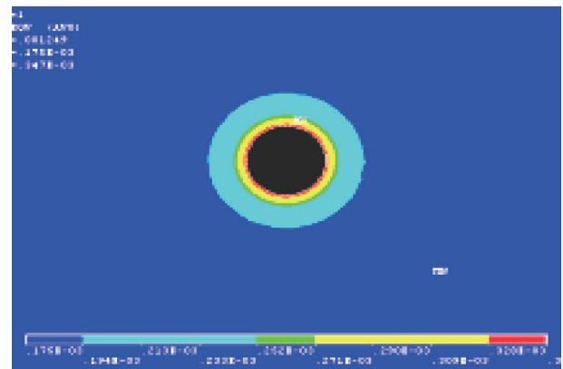
Figure 5 Finite Element Simulation Result of Fracturing Rock Stress Distribution
