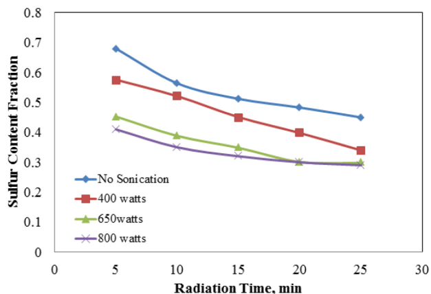
Figure 8 Role of Ultrasonic Wave Power on Percentage of Removed Sulfur
