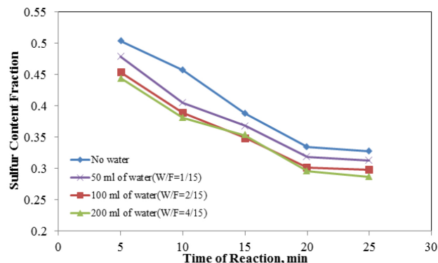
Figure 2 Role of Volume of Water Emulsified in 750 ml of Diesel on Desulfurization Process
