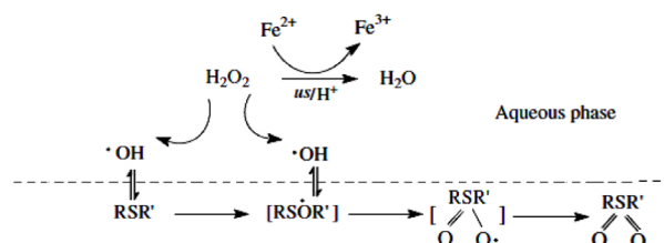
Figure 3 Possible Reaction Pathways for the Sulfur Compounds Oxidation Reaction in Ultrasound (Fe 2+ ) System [11]
