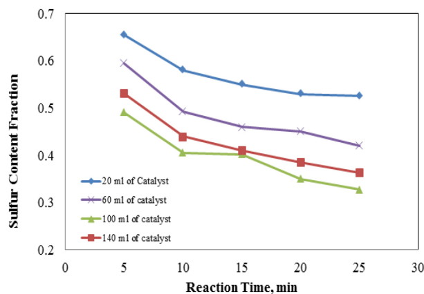
Figure 5 Percent of Removed Sulfur in Different Experiments with Fuel to Oxidant Ratio of 3:1
