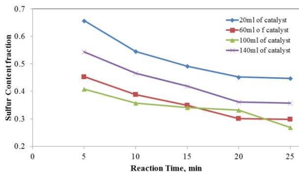
Figure 4 Percent of Removed Sulfur in Different Experiments with Fuel to Oxidant Ratio of 3:2
