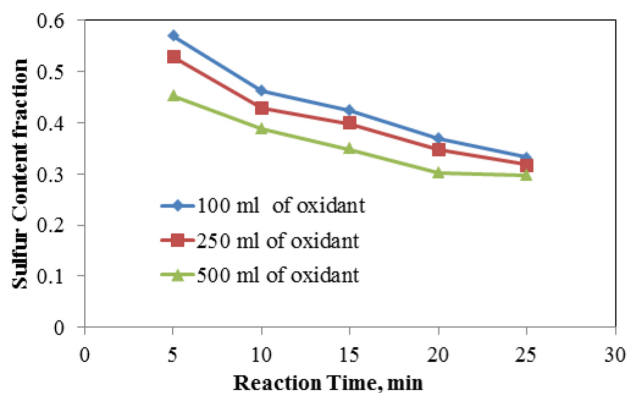
Figure 7 Percentage of Removed Sulfur at Different Times by Different Amount of Oxidant
