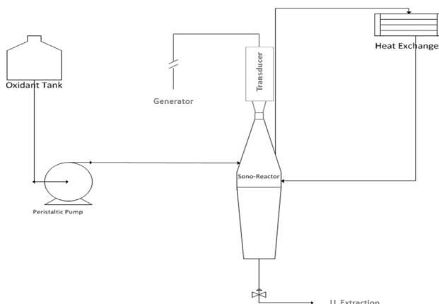
Figure 1 Schematic of Ultrasonic Assisted Oxidative Desulfurization Reactor
