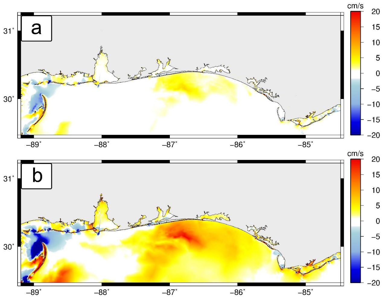
Figure 6.7: Changes in tidal velocities from the 2050 scenario for (a) the 2050-high scenario and (b) the 2100-high scenario; warm colors indicate tidal velocities have increased from the 2050 scenario, cool colors indicate tidal velocities have decreased from the 2050 scenario.
