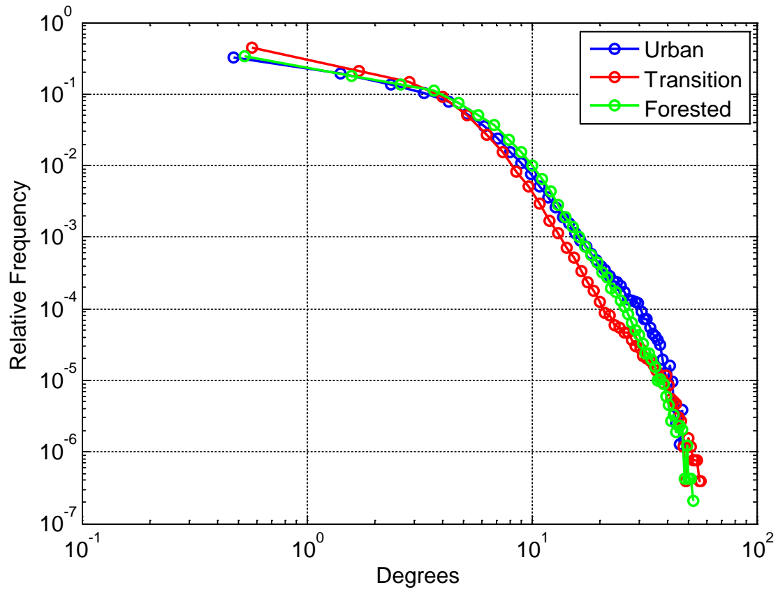
Figure 18 – Slope PDFs of the sample watersheds for each corresponding area. These particular basins are shown in Figure 2.
