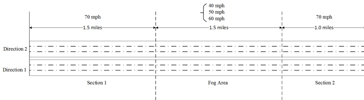
Figure 4-9 Experimental model setting
