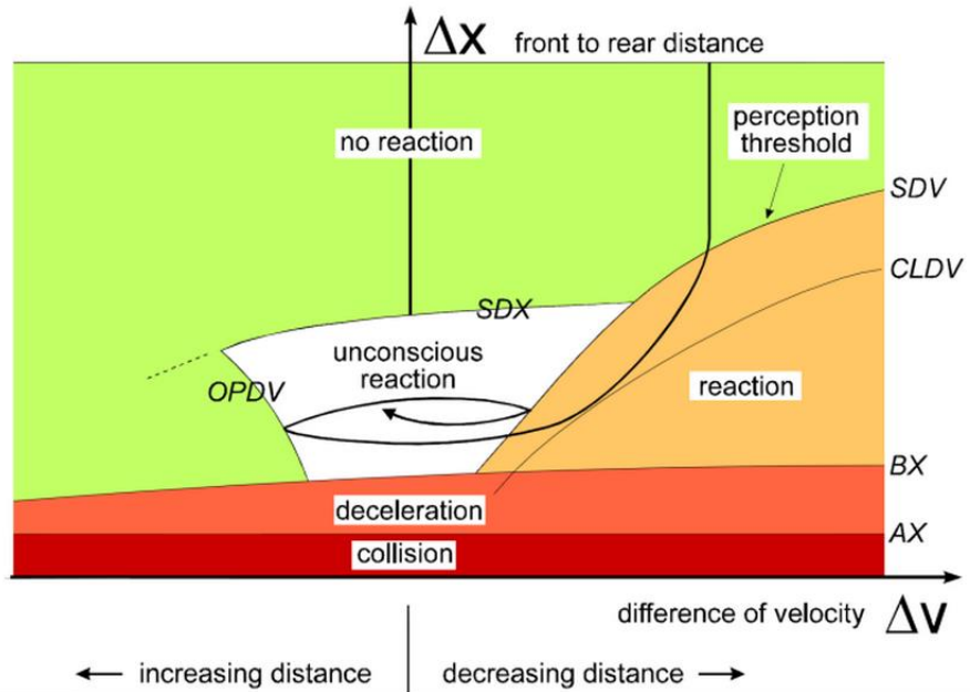
Figure 3-1 Wiedemann 1974 car following model
