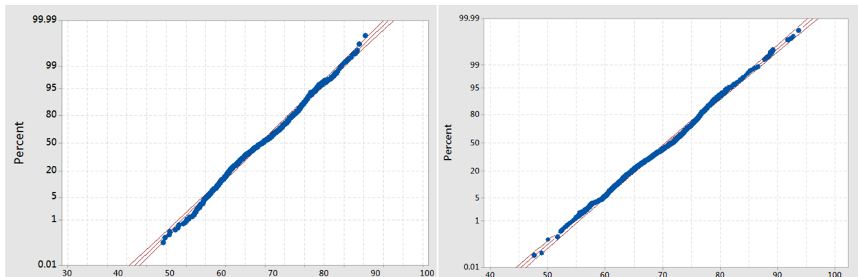
Figure 4-5 Probability plot of the speed of direction 1 and 2 in the field data
