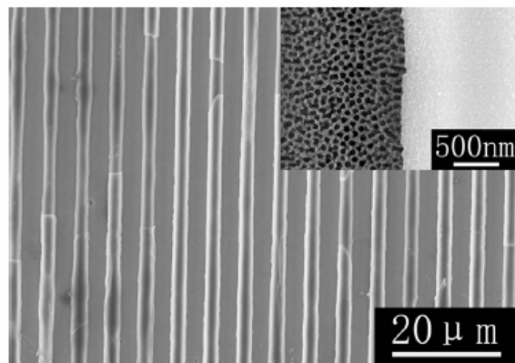
Figure 43. SEM Image of \text{SiO}_2 patterned aluminum oxide [26]
