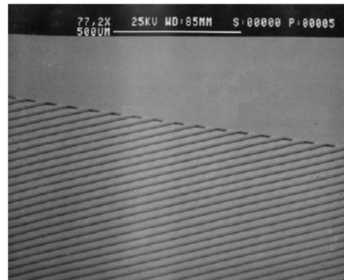
Figure 15. PMMA channels 5 \mu\text{m} deep [4]
