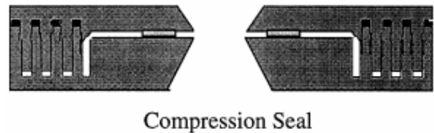
Figure 17. Interlocking finger joints with gasket closed [5]
