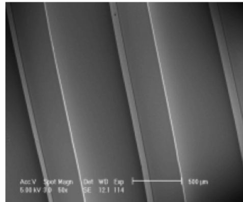
Figure 14. PMMA channels 250 \mu\text{m} deep [4]
