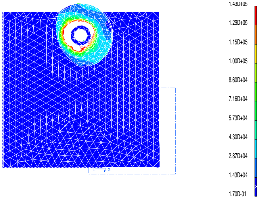
Figure 69. Finite Element Model of multiple-piece design (Front view)
