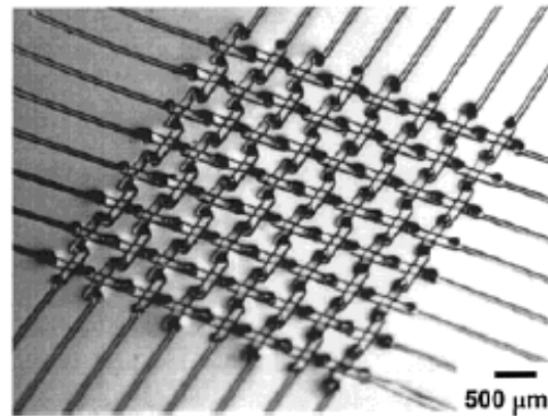
Figure 2. Optical micrograph of unenclosed lower membrane and microchannels in PDMS
