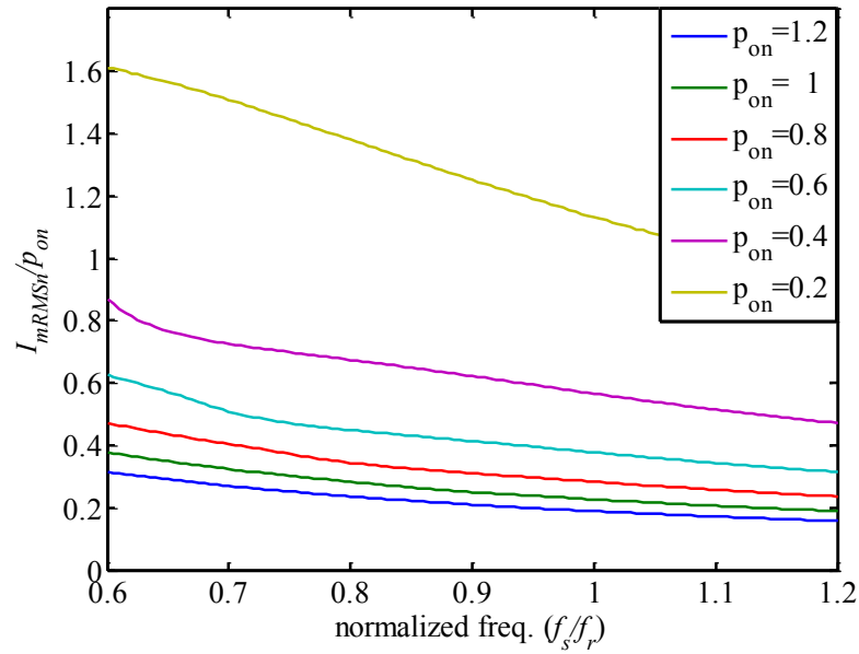
Figure 4.2 I_n/p_{on} under different frequency and load conditions
