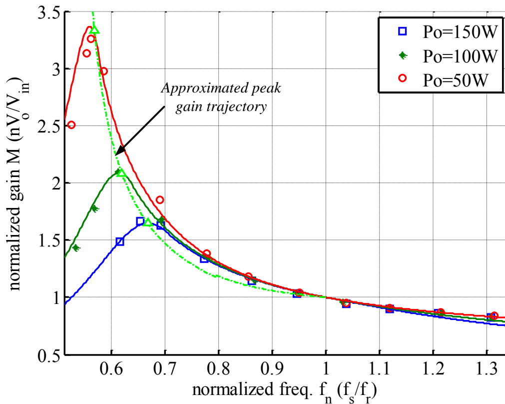
Figure 3.2 Gain curves obtained from mode analysis (solid lines), and experiment (markers), and estimated peak gain trajectory (dash-dot lines) with “ \Delta ” markers showing the estimated peak gain points at corresponding loads.
