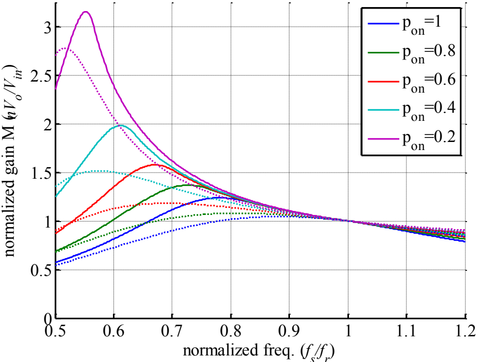
Figure 2.22 Gain curves comparison between mode analysis method (solid lines) and FHA method (dash lines) for m=4
