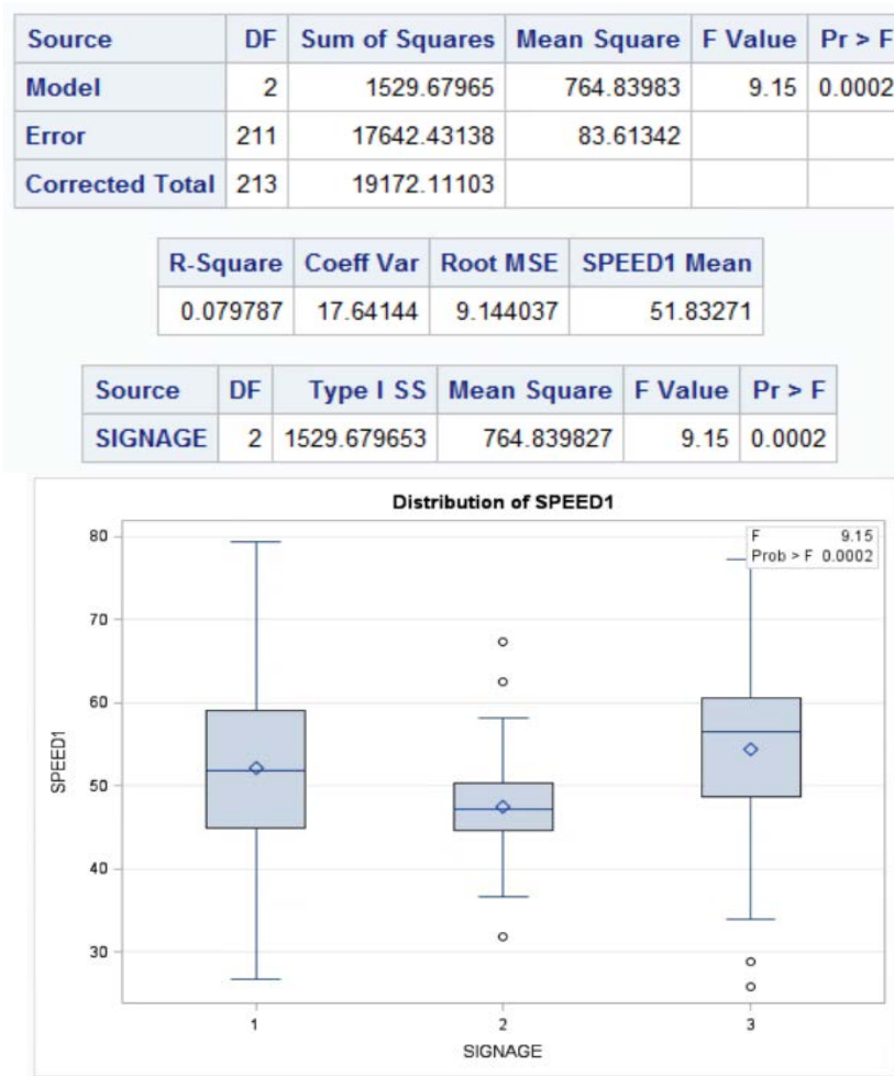
Figure 6 - 8. Signage boxplot for speed at location 1.
