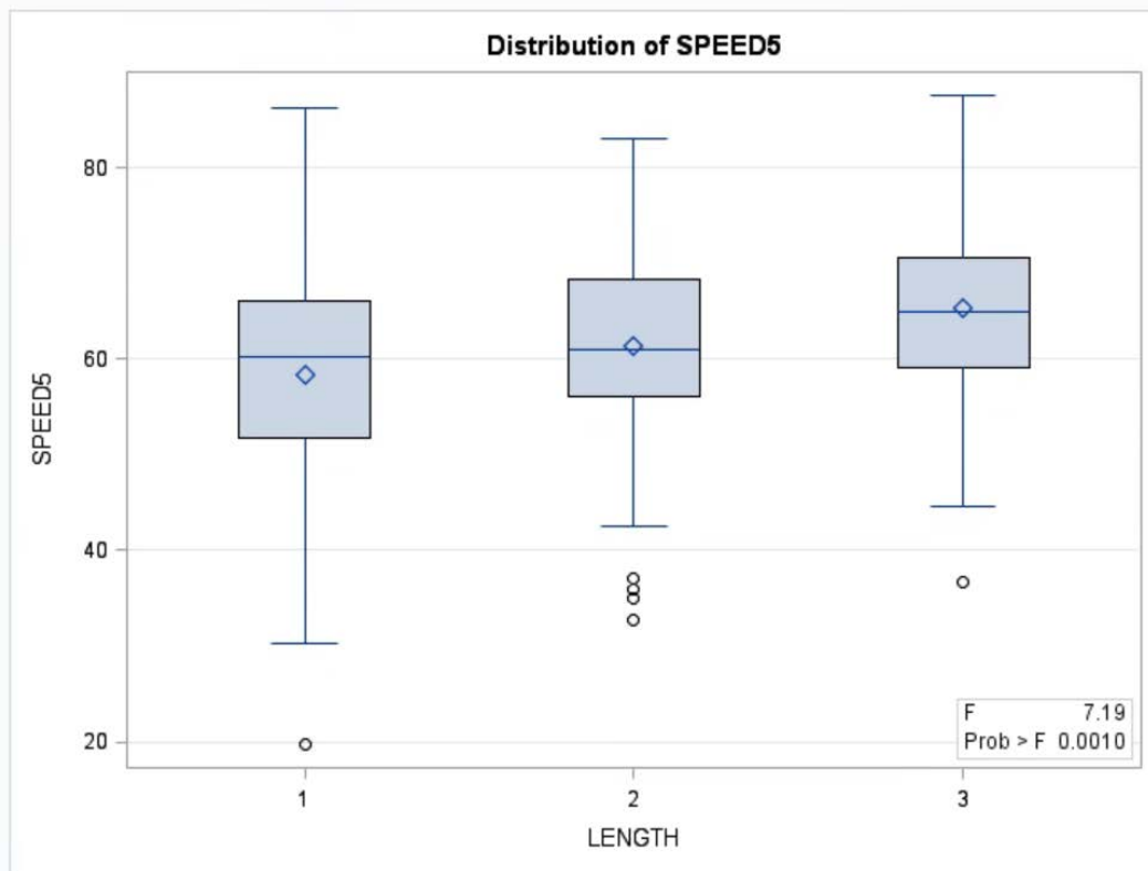
Figure 6 - 14. One-way ANOVA speed results for Length at location 5.
