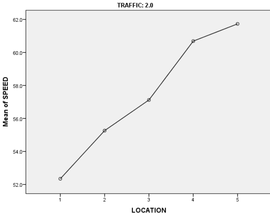
Figure 6 - 6. Mean peak hour speeds at each location.
