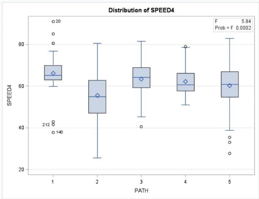
Figure 6 - 11. Boxplot of Path variable for speed at location 4.
