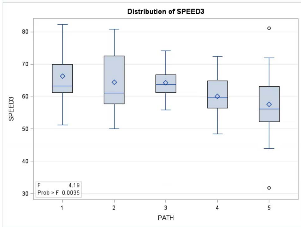
Figure 6 - 10. Graph of speed at location 3 for Path during off-peak.
