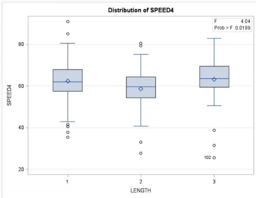
Figure 6 - 12. Boxplot of Length variable for speed at location 4.
