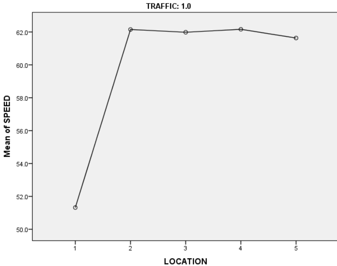
Figure 6 - 5. Mean off-peak hour speeds at each location.
