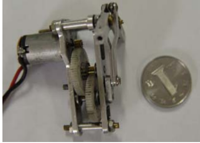
Fig. 3: The flapping mechanism
