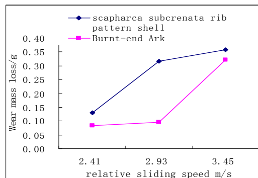
Fig. 8: The wear mass losses of Scapharca subcrenata node rib pattern shell and Burnt-end Ark shell
