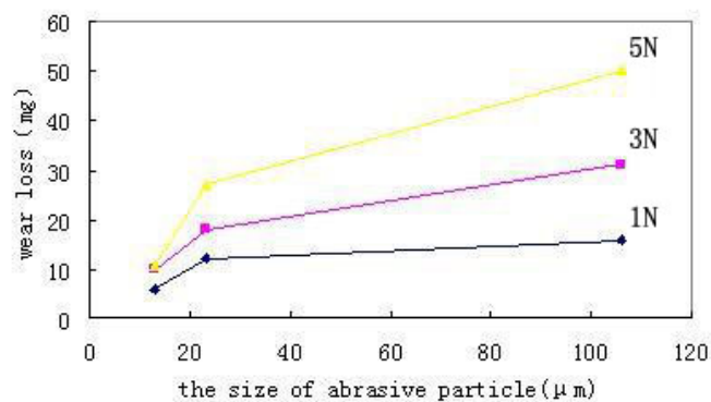
Figure 6: Wear of Haliotis discus hannai Ino shells under different loads
