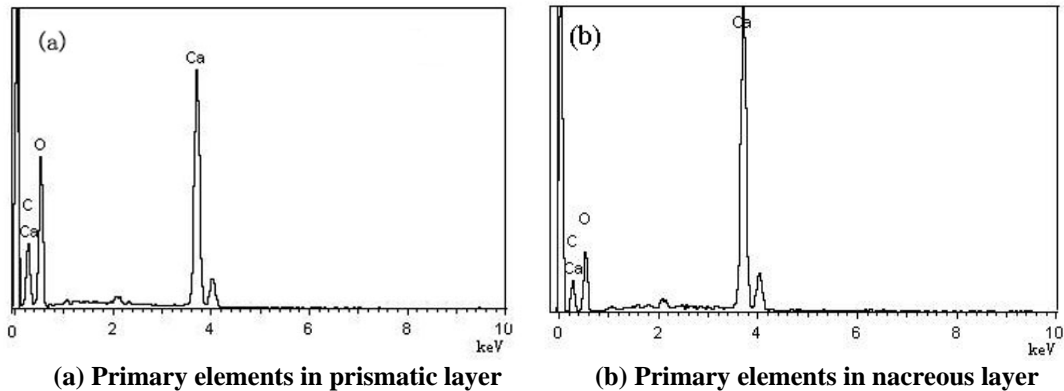
Figure 4: Primary elements in different layer
