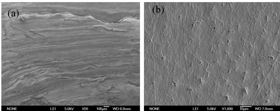
(a) The outer surface (b) The inner surface Figure 2: SEM surface morphologies of Haliotis discus hannai Ino shell
