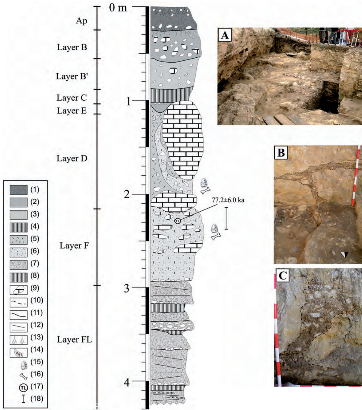
Fig. 2. Lithostratigraphic sequence of the Navalmaillo rockshelter. Legend and description: (1) Ap horizon. Limestone pebbles in silty sand matrix. Rootlets; (2) Limestone pebbles in silty carbonated matrix; (3) Limestone pebbles in silty matrix; (4) Silty clay; (5) Injected deposit with limestone cobbles in silty matrix; (6) At the top, limestone blocks and cobbles/pebbles in clay matrix. Abundant lithic and faunal remains; (7) Gravels of granitic and metamorphic rocks in sandy matrix; (8) Clay; (9) Limestone block; (10) Loading contact; (11) Bed contact; (12) Crossed stratification; (13) Rootlets; (14) Injection structures; (15) Lithic remains; (16) Faunal remains; (17) Thermoluminescence sample for dating. A. General view of the Navalmaillo rockshelter and B. and C. Detail of the level D.
