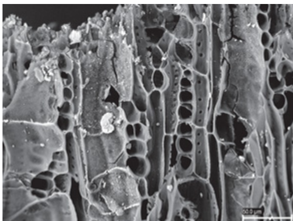
Fig. 6. SEM image of the Recouso charcoal sample (tangential section).
