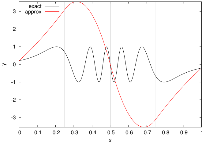
(a) Iteration 1. The solution is computed on a single four-element mesh. The red curve indicates the approximate solution, and the black line shows the exact analytic solution. The residue at element ( \rho_i in algorithm 2) exceeds the maximal residue times threshold \tau (here, fixed at 20%) only for the two central elements ( E_2 and E_3 ). The algorithm, therefore, decides to refine these two elements, which leads to the mesh shown in Figure 3b.
