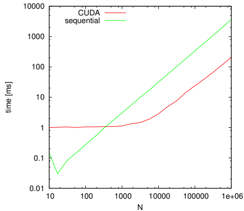
Figure 10. h-adaptation time for quadratic B-splines
