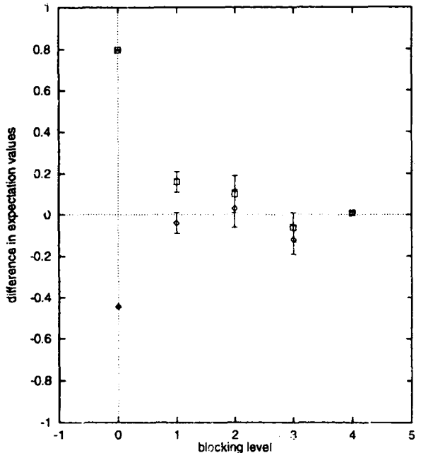
Fig. 4. This is the same plot as Fig. 2 except that O_1 is used instead of O_7 .
