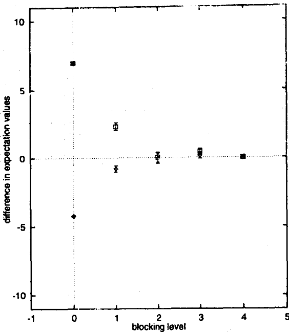
Fig. 2. The difference between expectation values of the maximum coordination number, O_7 , computed with two different actions as a function of the blocking level. The diamonds represent expectation values obtained with S = \alpha \sum_i \ln(q_i) minus those obtained with S = 0 when \alpha = +1 while the squares represent the analogous results for \alpha = -1 .
