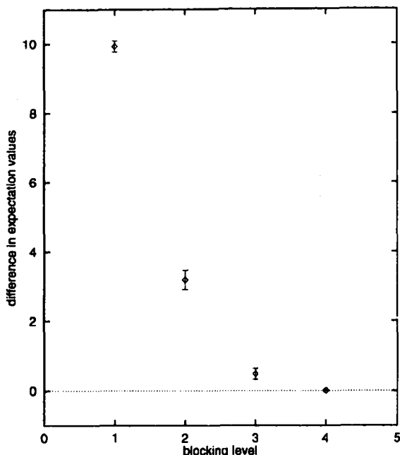
Fig. 1. The difference between expectation values of the maximum coordination number, O_7 , computed on lattices of the same size but for systems that differ (by one) in the number of times they have been blocked. The blocking level listed is that of the system that has been blocked the most. The original action is zero.
