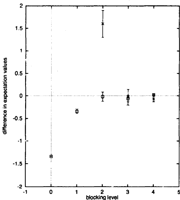
Fig. 5. This is the same plot as Fig. 3 except that O_1 is used instead of O_7 . Again, some of the \alpha = -10 data is off scale.
