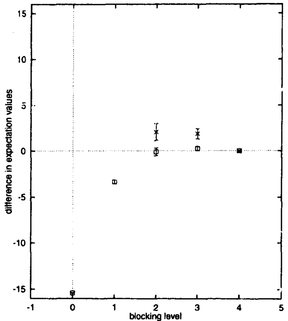
Fig. 3. This figure is like figure two except that the squares represent \alpha = +10 and the crosses represent \alpha = -10 . Crosses are missing for levels zero and one because the data is off scale by more than an order of magnitude.
