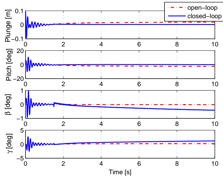
Figure 4.11: Open- and closed-loop system response under graded gust at pre-flutter speed V = 0.9V_f
