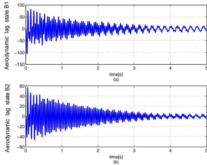
Figure 2.7: Open-loop aerodynamic lag states B_1, B_2 at post-flutter speed V = 1.2V_f
