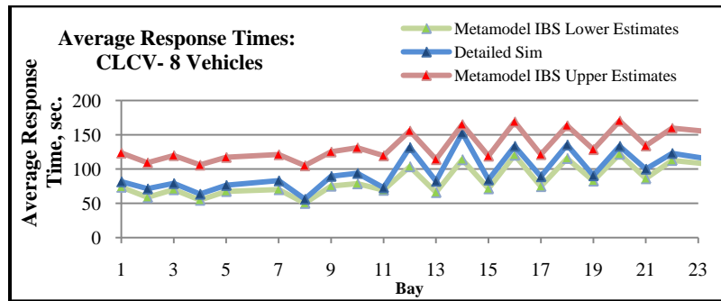
Figure 5-10: Response time to move requests for CLCV – 8 Vehicles
