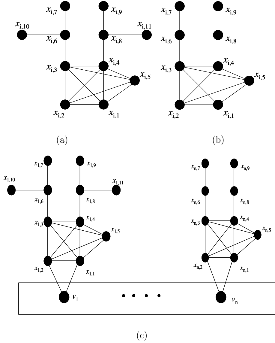
Figure 2.1: (a) An 11-vertex component (b) A 9-vertex component. (c) Constructed graph G' . Each vertex v_i , 1 \leq i \leq K is connected to an 11-vertex component and each vertex v_j , K + 1 \leq j \leq n , is connected to a 9-vertex component.
