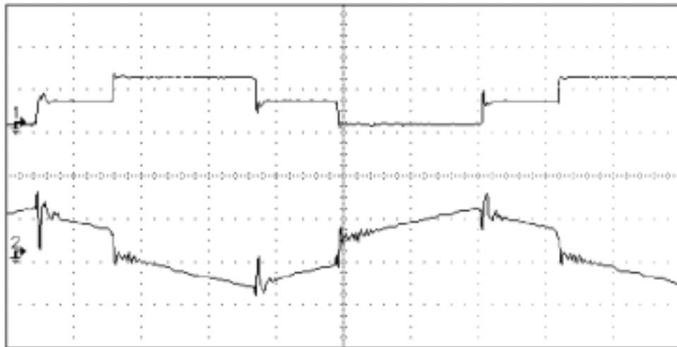
Fig. 5.22 Experimental waveforms of V_{ds} across low-side switch and transformer
