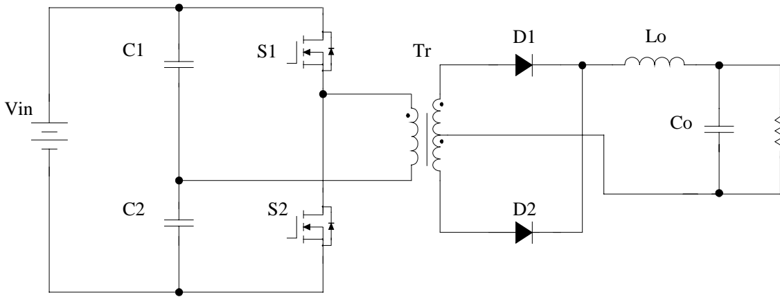
Fig. 4.1 Half-bridge topology
