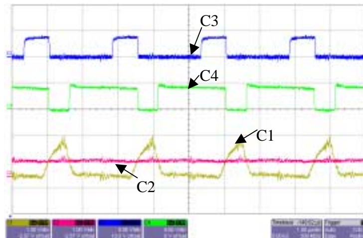
Fig. 3.20 The key waveform from the control board
