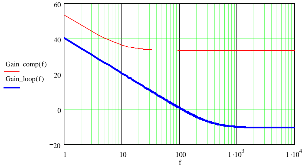
Fig. 4.7 (a) Gain
