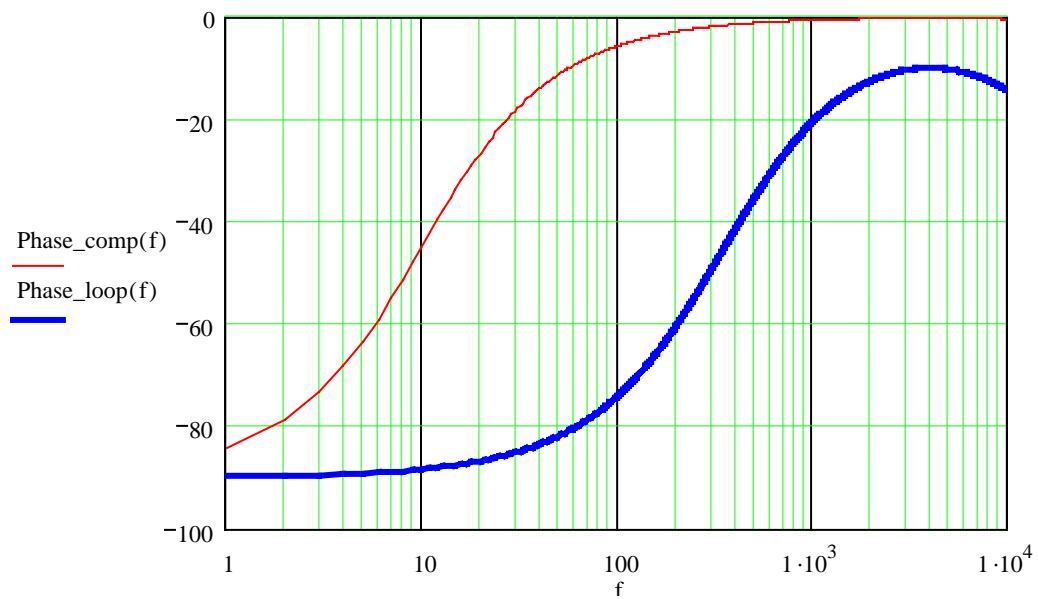
Fig. 4.7 (b) Phase
