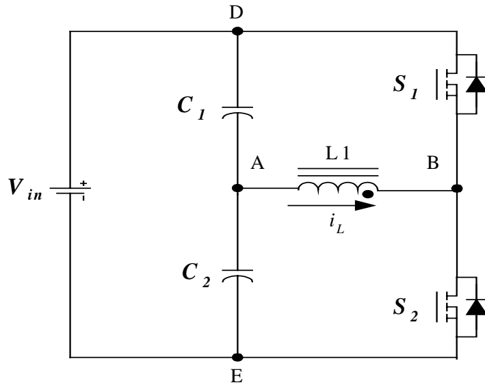
Fig. 3.3 Half-Bridge topology
