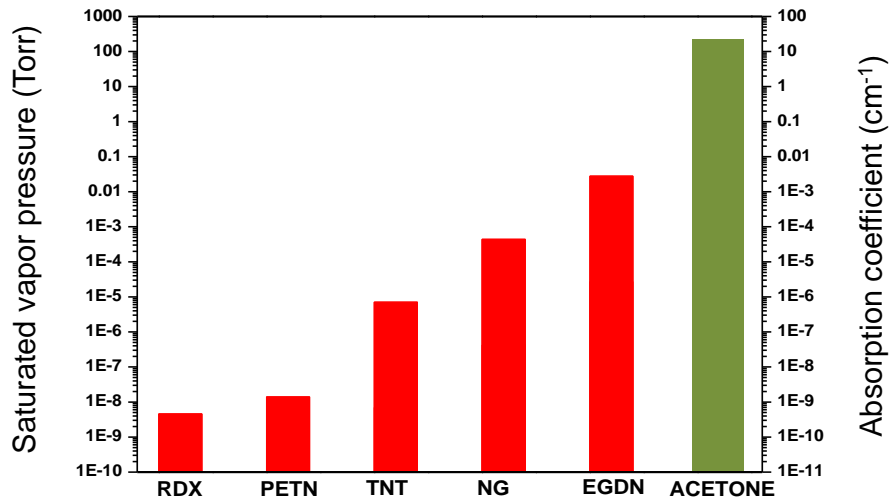
Figure 1.2 : Saturated vapor pressures and absorption coefficients of a few common explosives compared with acetone.
