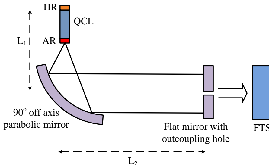
Figure 6.1 : Schematic of an external cavity QCL at 8.1 \mu\text{m} . The transmitted spectrum of the external cavity was measured using Fourier spectrometer (FTS).
