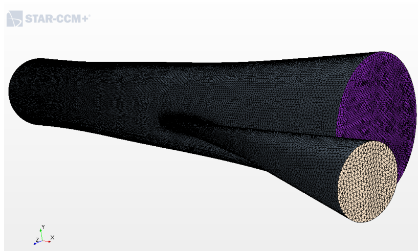
Figure 49: Simplified IJS 3D Geometry for CFD.
