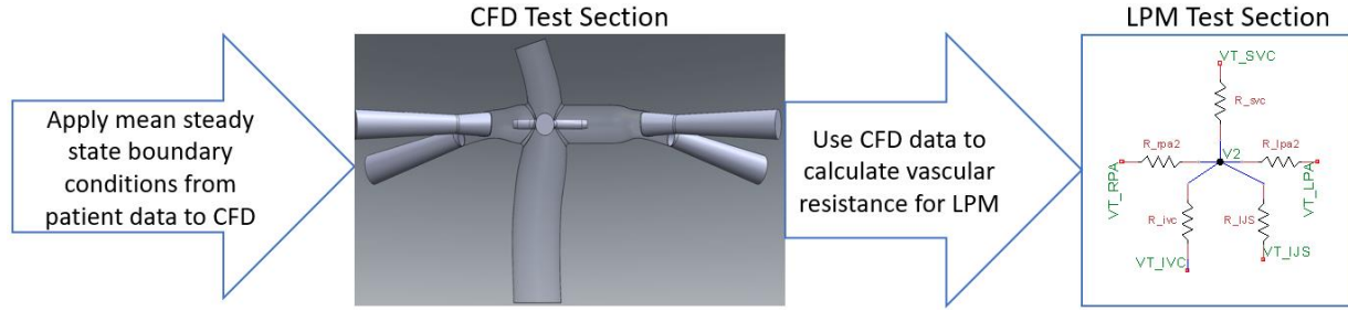
Figure 23: LPM Test Section Initialization.
