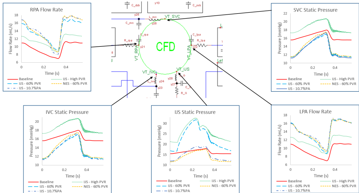
Figure 56: Synthetic Model: Converged CFD Boundary Conditions.
