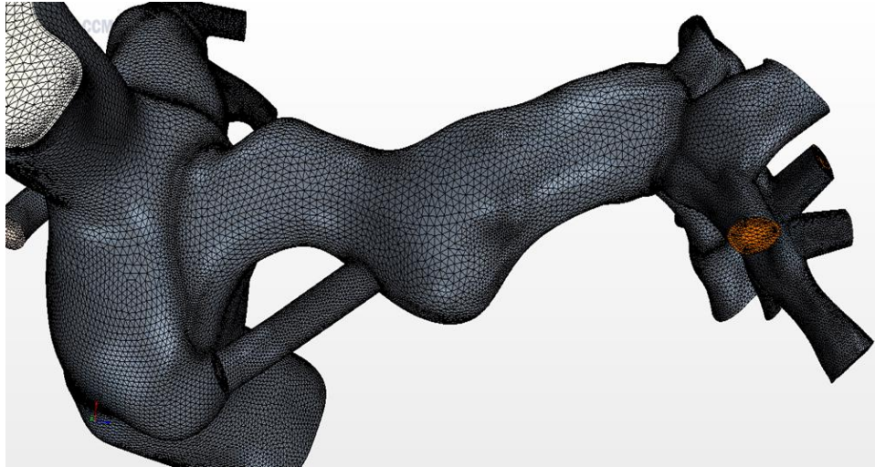
Figure 25: Tetrahedral Mesh of the CHOP-1 Model.
