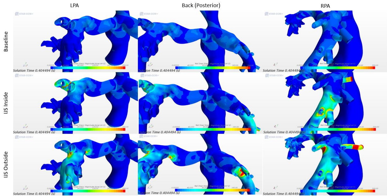
Figure 73: CHOP-1 Model: Wall Shear Stress at Peak Systole.
