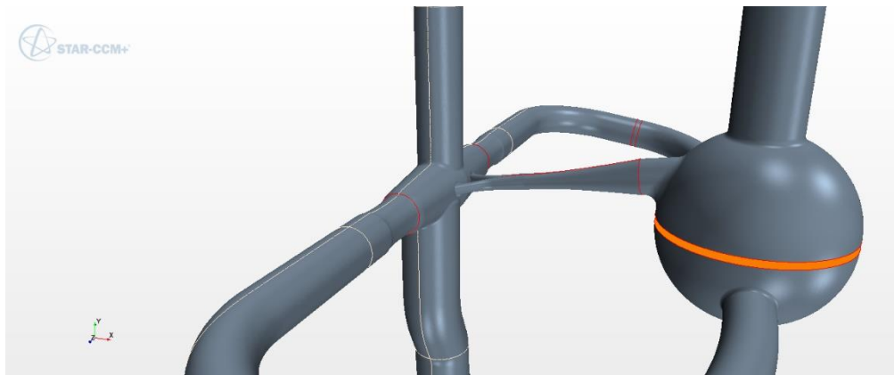
Figure 41: Offset of the IVC by 50% toward the LPA.
