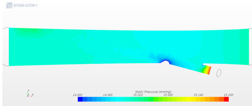
Figure 35: Contours of Static Pressure – Inner IJS.
