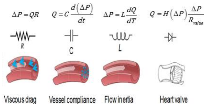
Figure 20: Hydraulic Analogy.
