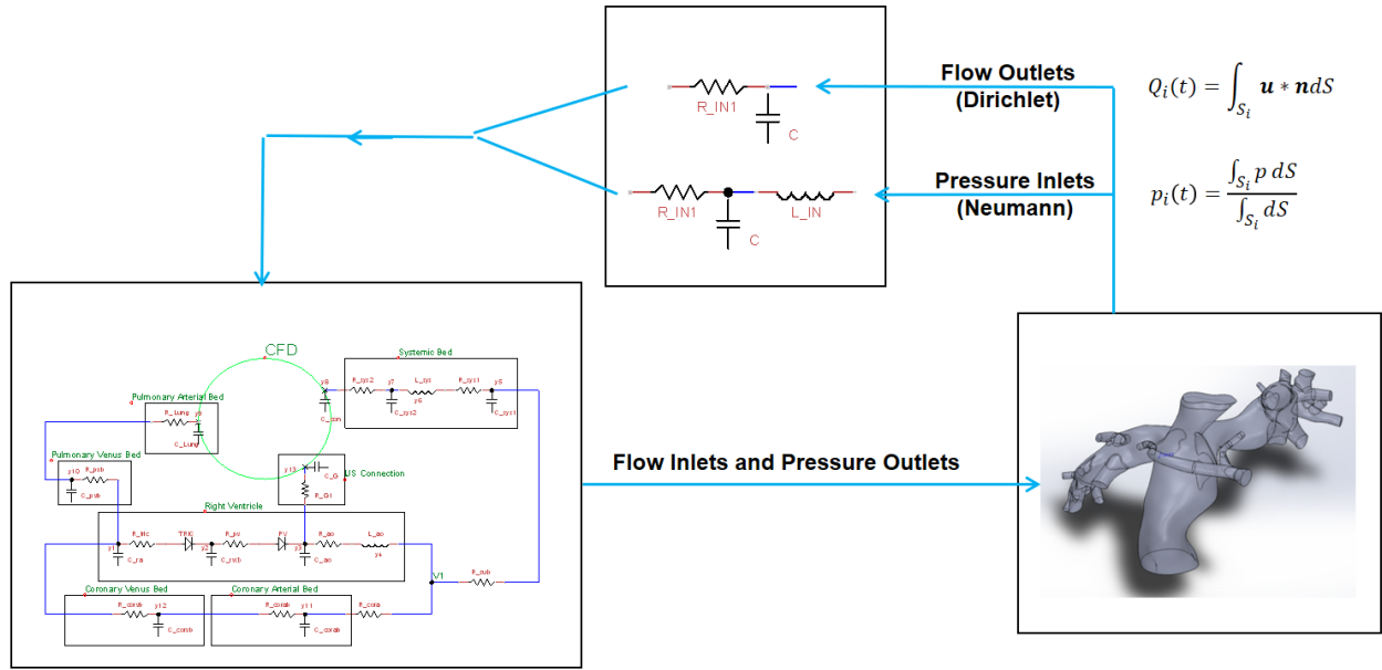
Figure 28: Interface Parameter Selection. Q: Flow Rate, p: Pressure, u: Velocity Vector, n: Normal Surface, S: Surface.
