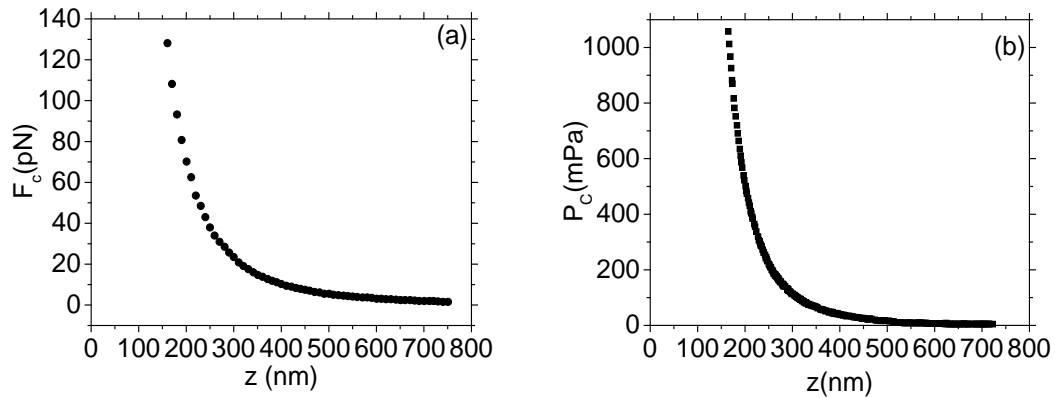
Figure 8: (a) Measured magnitude of F_c(z) with respect to the separation of the sphere-plate configuration. (b) Determine magnitude of P_c(z) between parallel plates using the sphere-plate configuration [10].
