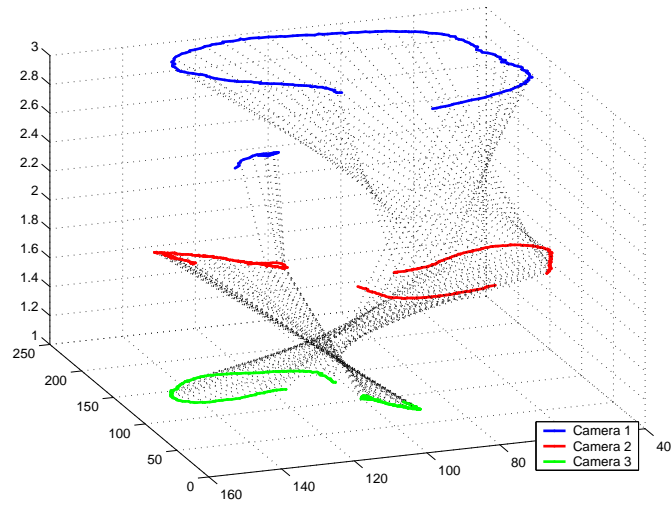
Figure 4.12: Correspondence across the 3 moving cameras. For each sequence, each pair of tracks is plotted at a level. The point-wise correspondence is show by the dotted black line.
