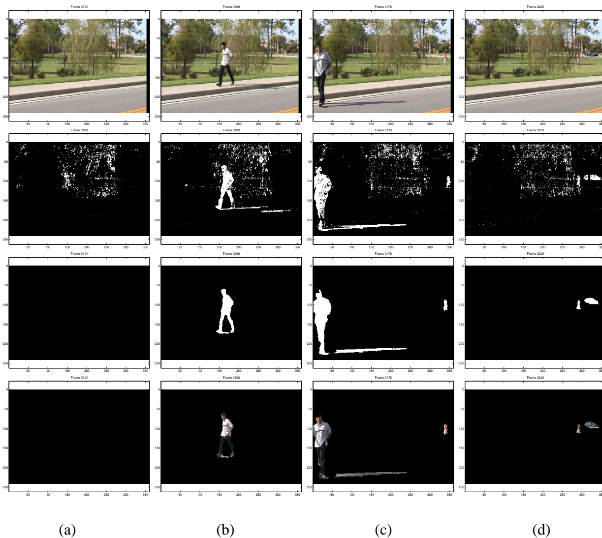
Figure 3.11: Swaying trees sequence. A weeping willow sways in the presence of a strong breeze. The top row shows the original images, the second row are the results obtained by using the mixture of Gaussians method, and the third row are the results obtained by our method. The fourth row is the masked original image. Morphological operators were not used in the results.
