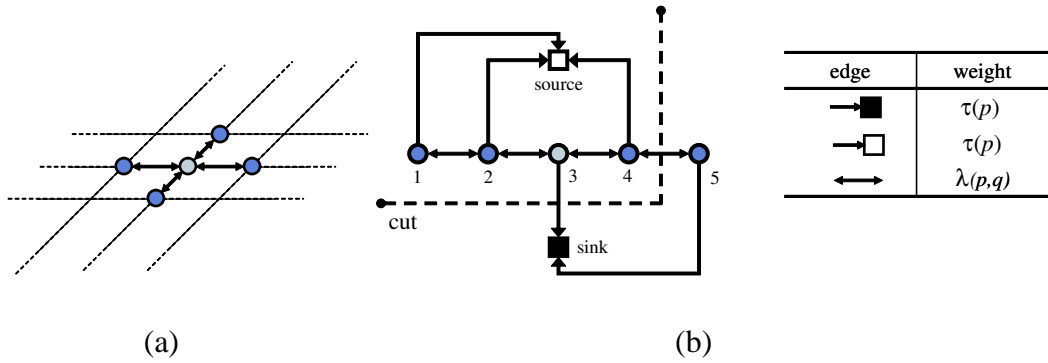
Figure 3.5: A 4-neighborhood system. Each pixel location corresponds to a node in the graph, connected by a directed edge to the source and the sink, and by an undirected edge to its four neighbors. For purposes of clarity the edges between node 3 and nodes 5 and 1 have been omitted in (b).
