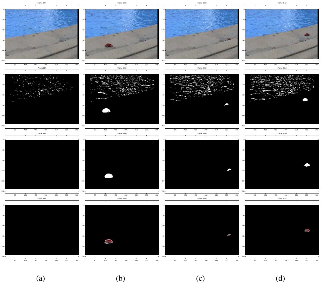
Figure 3.8: Poolside sequence. The water in this sequence shimmers and ripples causing false positive in conventional detection algorithms, as a remote controlled car passes on the side. The top row are the original images, the second row are the results obtained by using a 5-component, Mixture of Gaussians method, and the third row are the results obtained by our method. The fourth row is the masked original image. Morphological operators were not used in the results.
