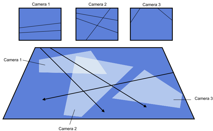
Figure 5.1: A unified framework for estimating inter-camera transformations. Overlapping and non-overlapping views are handled identically, since we look at global object motion models rather than pairwise correspondences.
