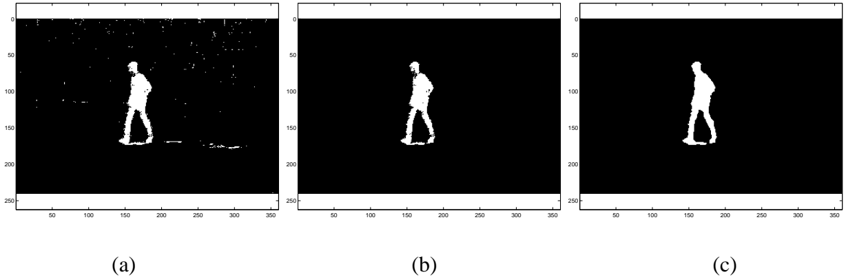
Figure 3.4: Three possible detection strategies. (a) Detection by thresholding using only the background model of Equation 3.1. Noise can cause several spurious detections. (b) Detection by thresholding the Likelihood Ratio of Equation 3.8. Since some spurious detections do not persist in time, false positives are reduced using the foreground model. (c) Detection using MAP-MRF estimation, 3.13. All spurious detections are removed and false negative within the detected object are also removed as a result of their spatial context.
