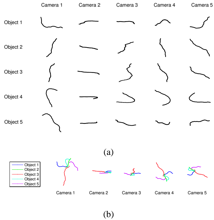
Figure 4.7: Data generation. The randomly generated data captures the smoothness of real trajectories. There are 5 cameras observing 5 objects, for 100 frames. The mean of motion magnitude, \bar{\rho} was set to 50, the noise variance, \sigma_\epsilon was 2. (a) 5 objects viewed in 5 cameras. Each row corresponds to the image of the trajectory in that camera. (b) The image of all objects in each camera, with trajectories color-coded for association.
