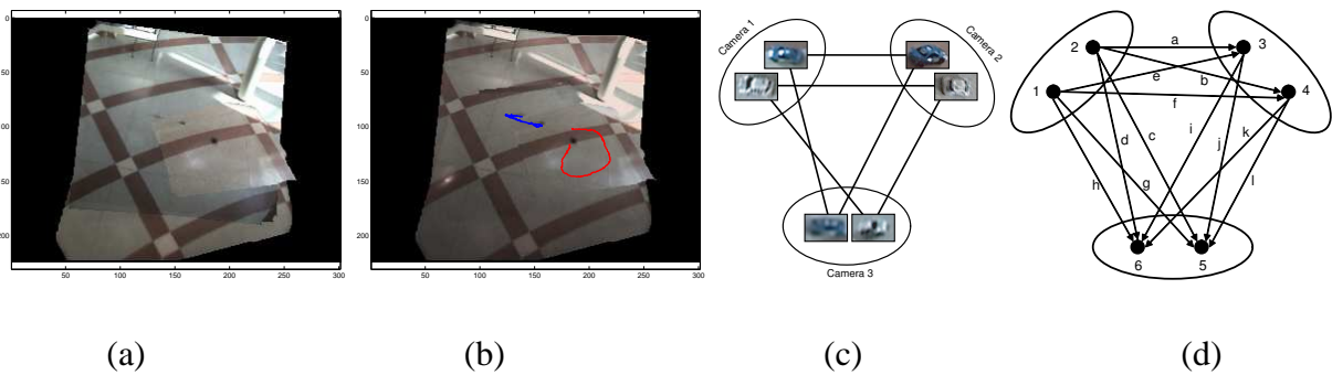
Figure 4.11: Concurrent visualization of three sequences. (a) Concurrent mosaic before blending, (b) Blended concurrent mosaic with the track overlaid. Matching in three sequences. (c) Matching of the tripartite graph, (d) The corresponding directed graph.
