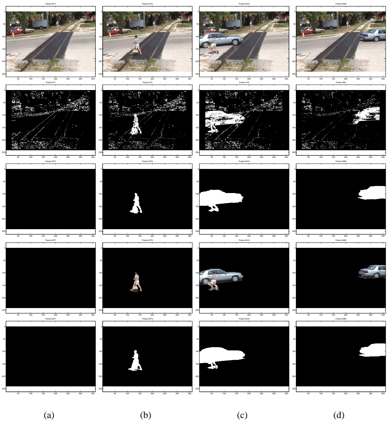
Figure 3.7: Background Subtraction in a nominally moving camera (motion is an average of 12 pixels). The top row are the original images, the second row are the results obtained by using a 5-component, Mixture of Gaussians method, and the third row results obtained by our method. The fourth row is the masked original image. The fifth row is the manual segmentation. Morphological operators were not used in the results.
