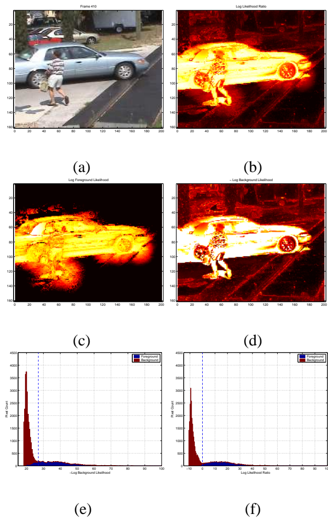
Figure 3.3: Improvement in discrimination using temporal persistence. Whiter values correspond to higher likelihoods of foreground membership. (a) Video Frame 410 of the Nominal Motion Sequence (b) Log-Likelihood Ratio values obtained using Equation 3.8. (c) Foreground likelihood map. (d) Background negative log-likelihood map. (e) Histogrammed negative log-likelihood values for background membership. The dotted line represents the ‘natural’ threshold for the background likelihood, i.e. \log(\gamma) . (f) Histogrammed log-likelihood ratio values. Clearly the variance between clusters is decidedly enhanced. The dotted line represents the ‘natural’ threshold for the log-likelihood ratio, i.e. zero.
