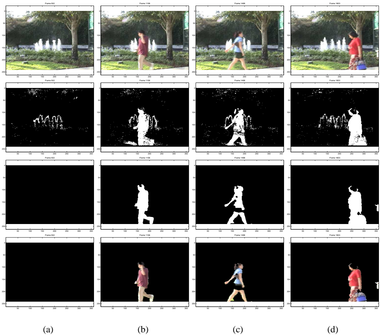
Figure 3.9: Fountain Sequence. Background Subtraction in the presence of dynamic textures. There are three sources of nonstationarity: (1) The tree branches oscillate (2) The fountains (3) The shadow of the tree on the grass below. The top row are the original images, the second row are the results obtained by using a 5-component, Mixture of Gaussians method, and the third row results obtained by our method. The fourth row is the masked original image. Morphological operators were not used in the results.
