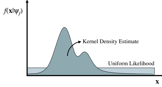
Figure 3.2: Foreground likelihood function. The foreground likelihood estimate is a mixture of the kernel density estimate and a uniform likelihood across the 5-space of features. This figure shows a conceptualization as a 1-D function.
