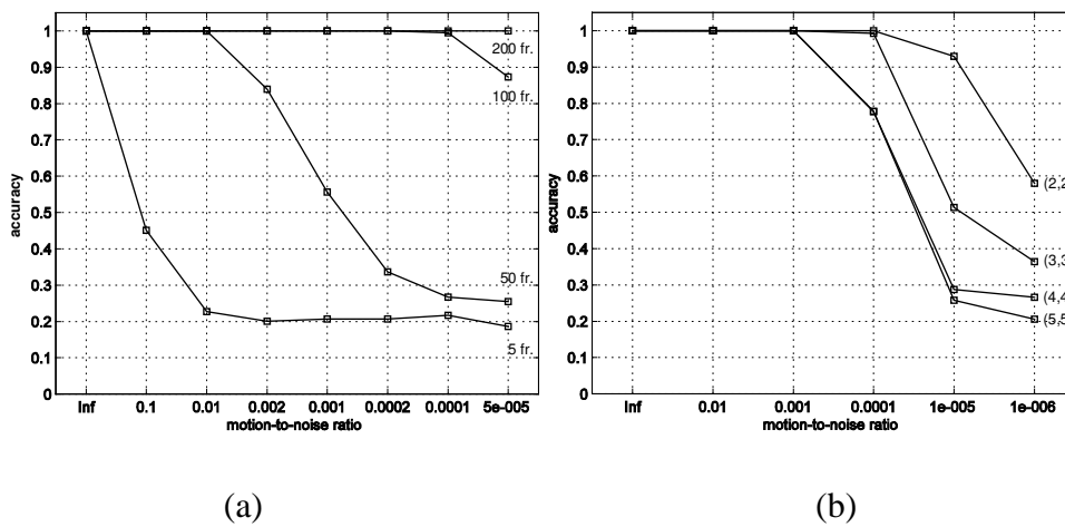
Figure 4.9: Association accuracy w.r.t number of cameras, number of objects, number of frames and motion-to-noise ratio. Note: the horizontal axis is not progressing linearly. (a) For ten cameras with ten objects the percentage of correct associations to the total number of associations. (b) As the number of cameras and objects increase linearly, for a fixed 60 frames, the association accuracy decreases. The results are the average of 100 runs.
