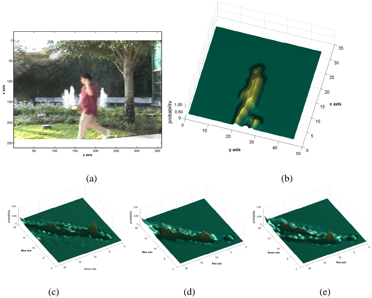
Figure 3.1: Foreground Modeling. Using kernel density estimates on a model built from recent frames, the foreground can be detected in subsequent frames using the property of temporal persistence, (a) Current Frame (b) the X, Y -marginal, f_{X,Y}(x, y) . High membership probabilities are seen in regions where foreground in the current frame matches the recently detected foreground. The non-parametric nature of the model allows the arbitrary shape of the foreground to be captured accurately (c) the B, G -marginal, f_{B,G}(b, g) (d) the B, R -marginal, f_{B,R}(b, r) (e) the G, R -marginal, f_{G,R}(g, r) .
