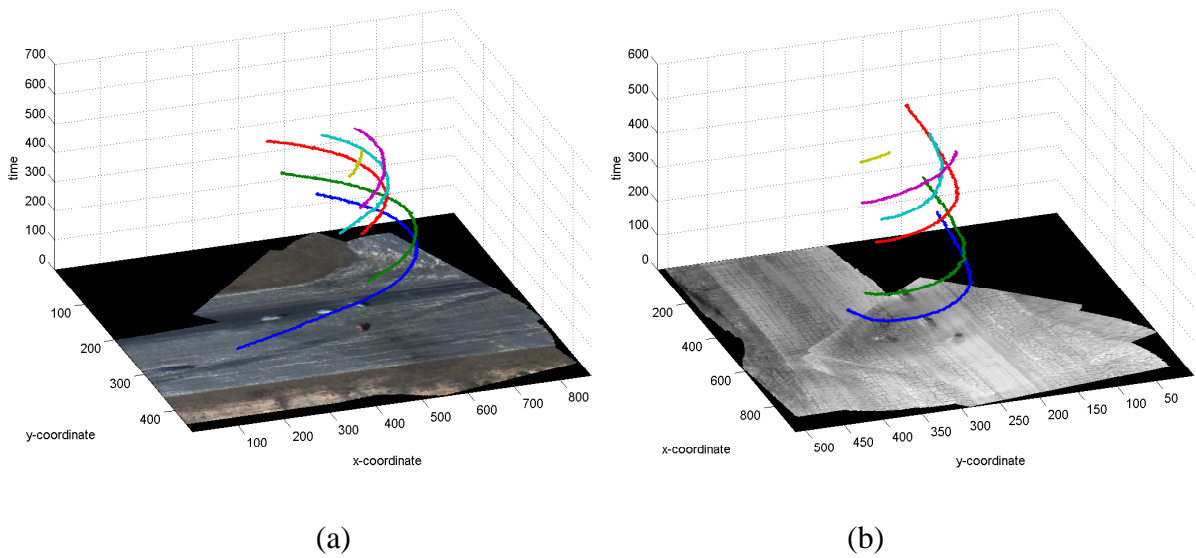
Figure 4.15: First UAV Experiment - two cameras, six objects. (a) The EO video, (b) The IR video. Since we are using only motion information, association can be performed across different modalities.
