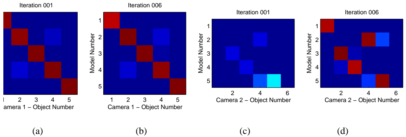
Figure 5.6: Adjacency matrix across EM Iterations containing the probabilities of association. (a) Adjacency Matrix at the first iteration between Camera 1 and the model lines, (b) Adjacency Matrix at the after convergence (6 iterations) (c) Adjacency Matrix at the first iteration between Camera 2 and the model lines, (d) Adjacency Matrix at the after convergence (6 iterations).
