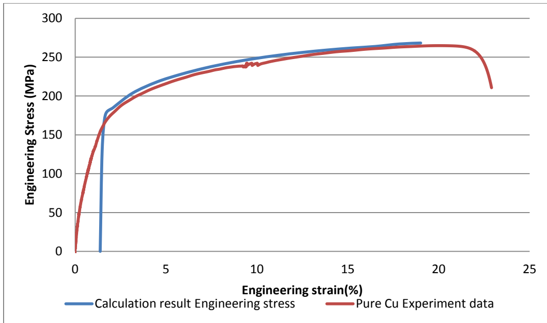
Figure 14 Engineering stress strain of pure copper calculation Vs Experiment
