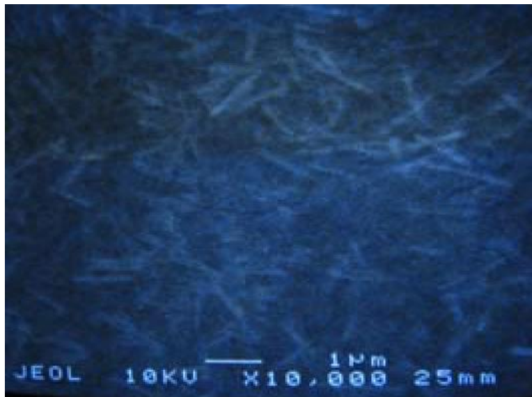
Figure 5 SEM picture of Cu/CNT composites Composites is fabricated by the electrochemical co-deposition[147]
