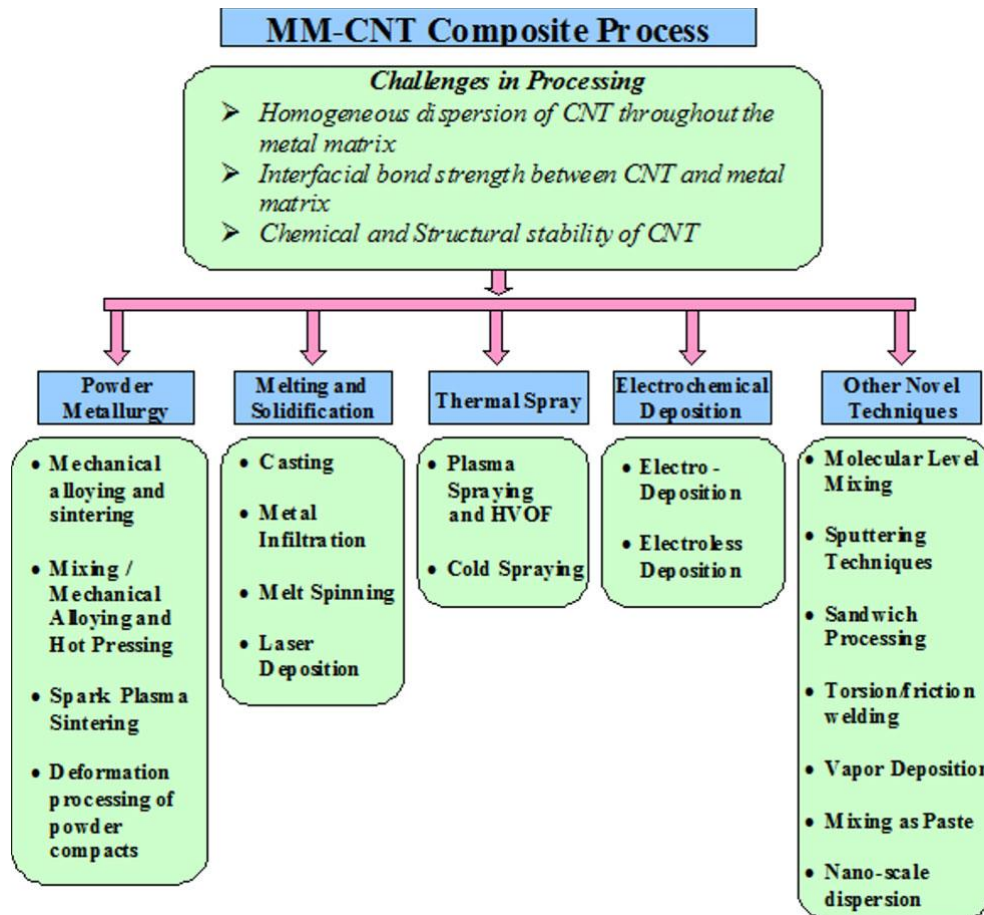
Figure 3 Metal matrix CNTs composite processing Several metal matrix CNT composites methods are presented[41]
