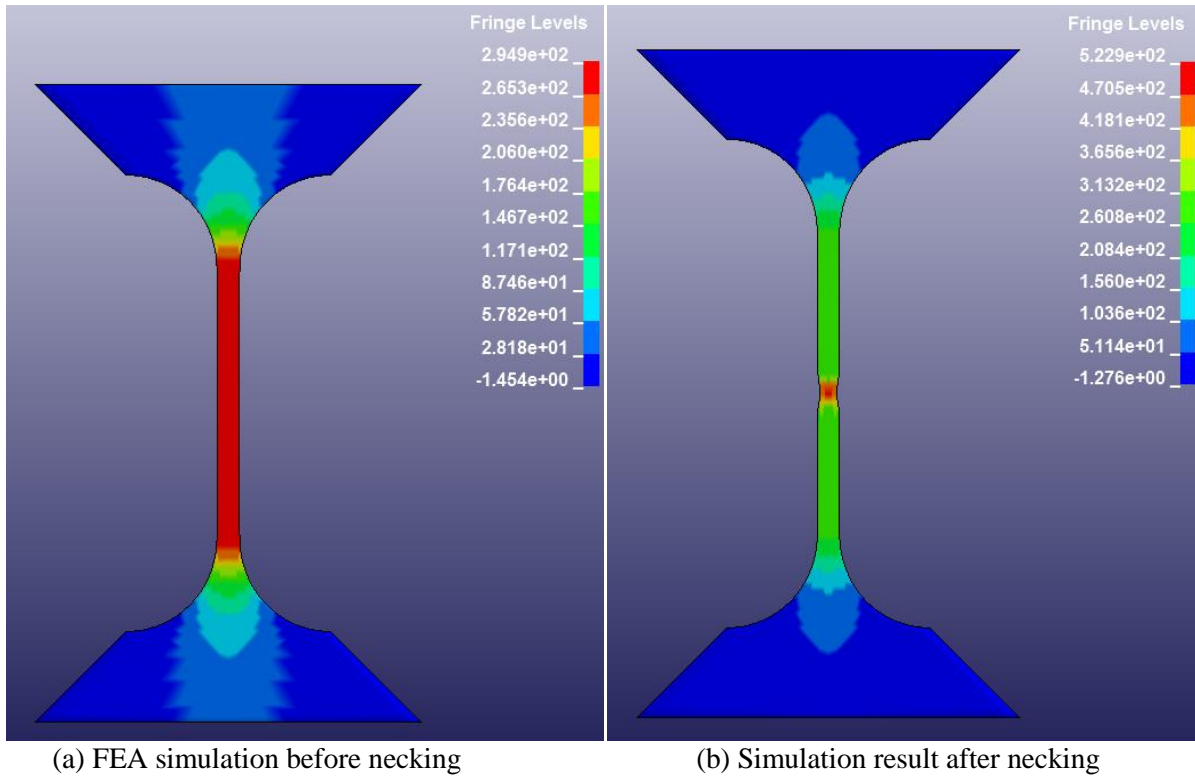
Figure 19 Plastic strain contour plot of meshing 1
