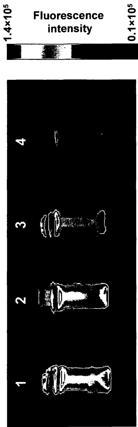
1. Control; 2. 1 \mu\text{M} \text{H}_2\text{O}_2 ; 3. 6 \mu\text{M} \text{H}_2\text{O}_2 ; 4. 6 \mu\text{M} \text{H}_2\text{O}_2 (pH 4.0)
