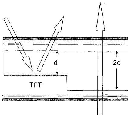
Fig. 1b Double Cell Gap (PRIOR ART)
