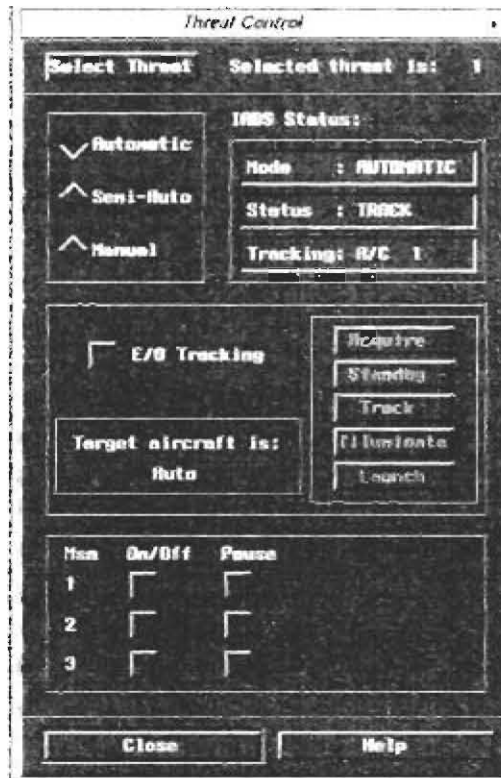
Figure 6-18. The Threat Control panel.
