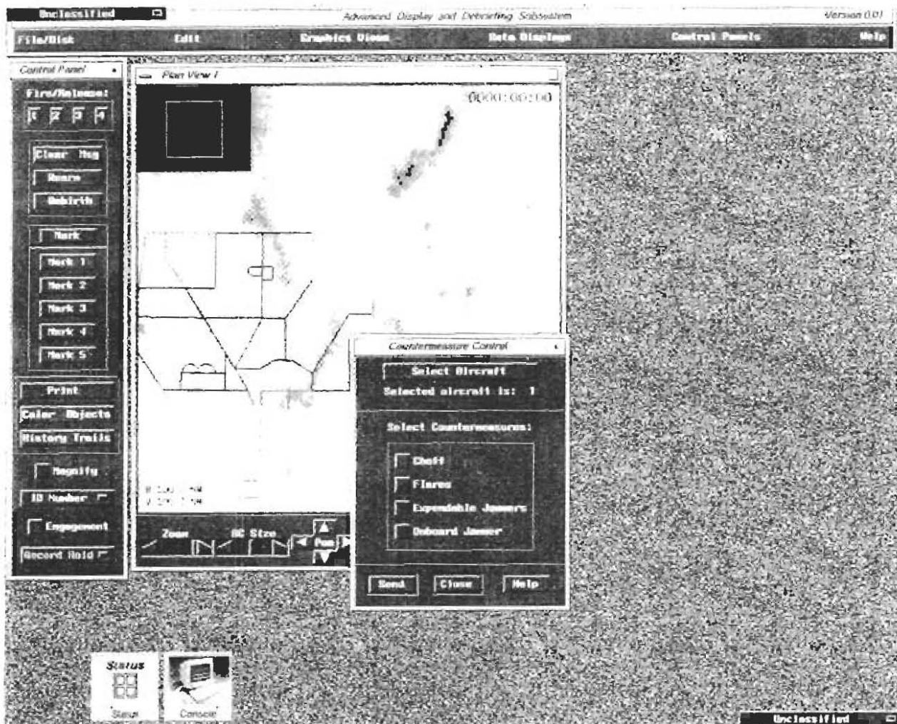
Figure 7-22. Countermeasures Control Panel occluding the Plan View display.
