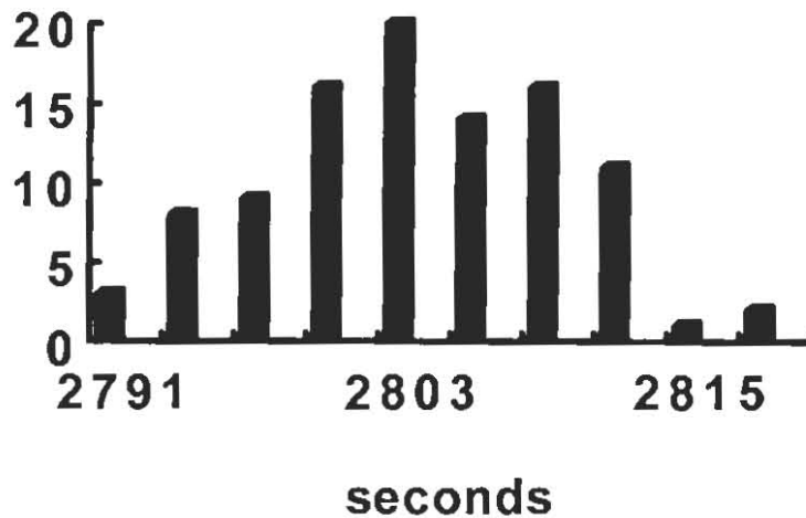
Figure 5-1. Distribution of times for making 512 pairings per the ADDS design specification.
