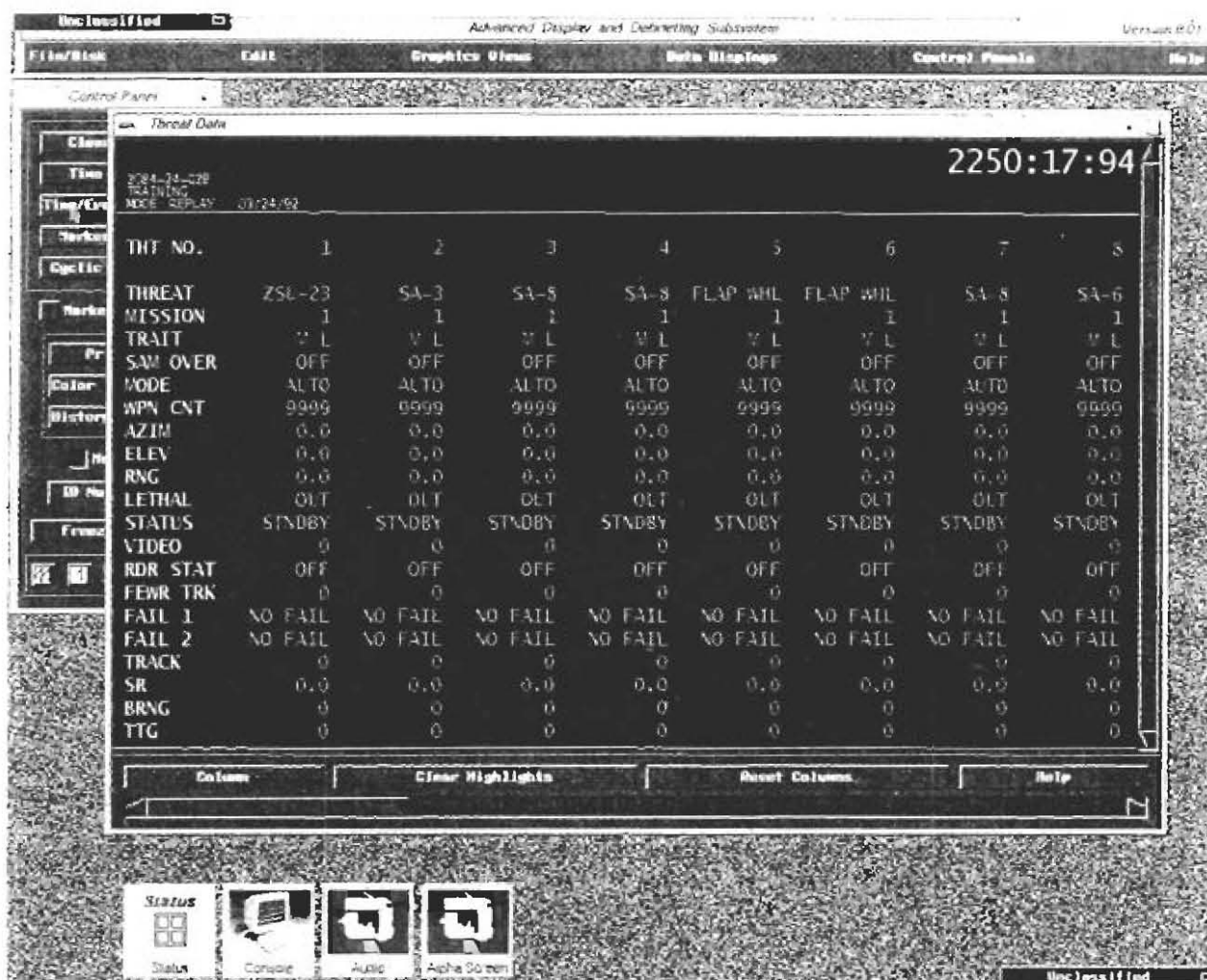
Figure 7-18. Threat Data display.
