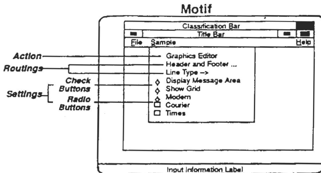
Figure A5-4. Example of an action menu entry.
