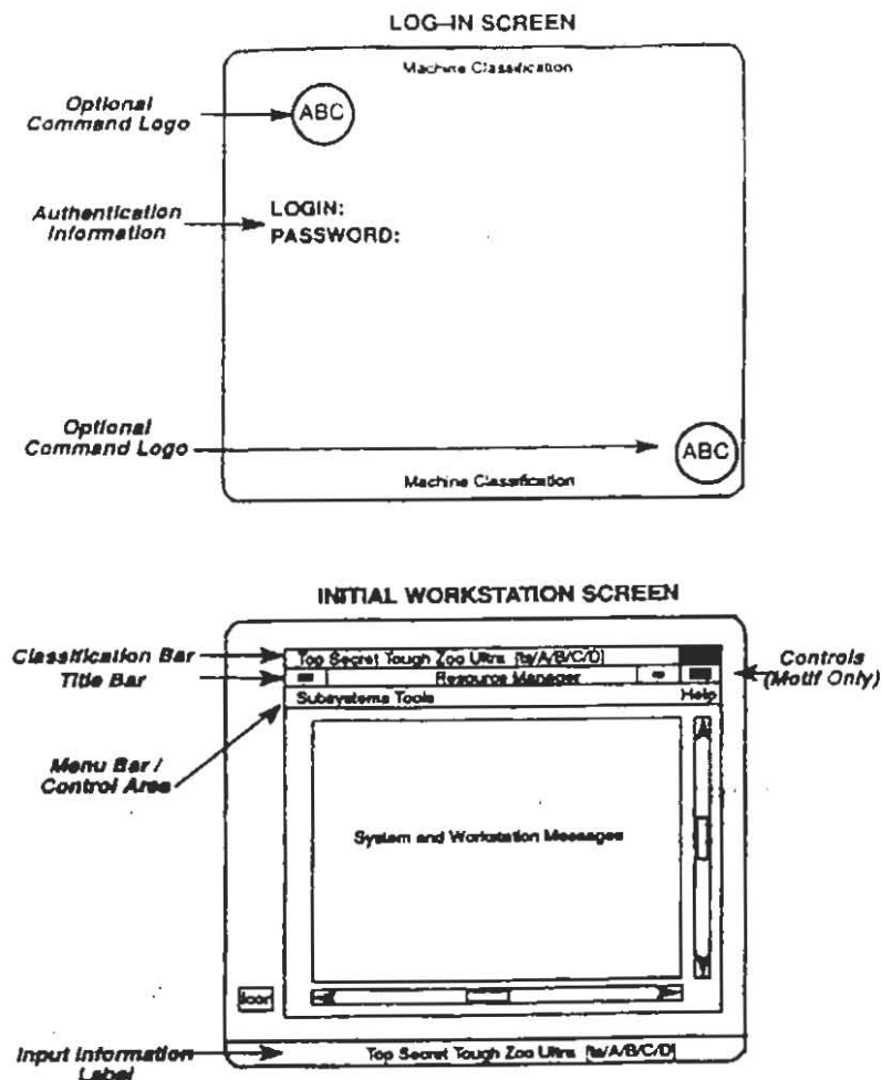
Figure A4-1. Example of a log-in screen.
