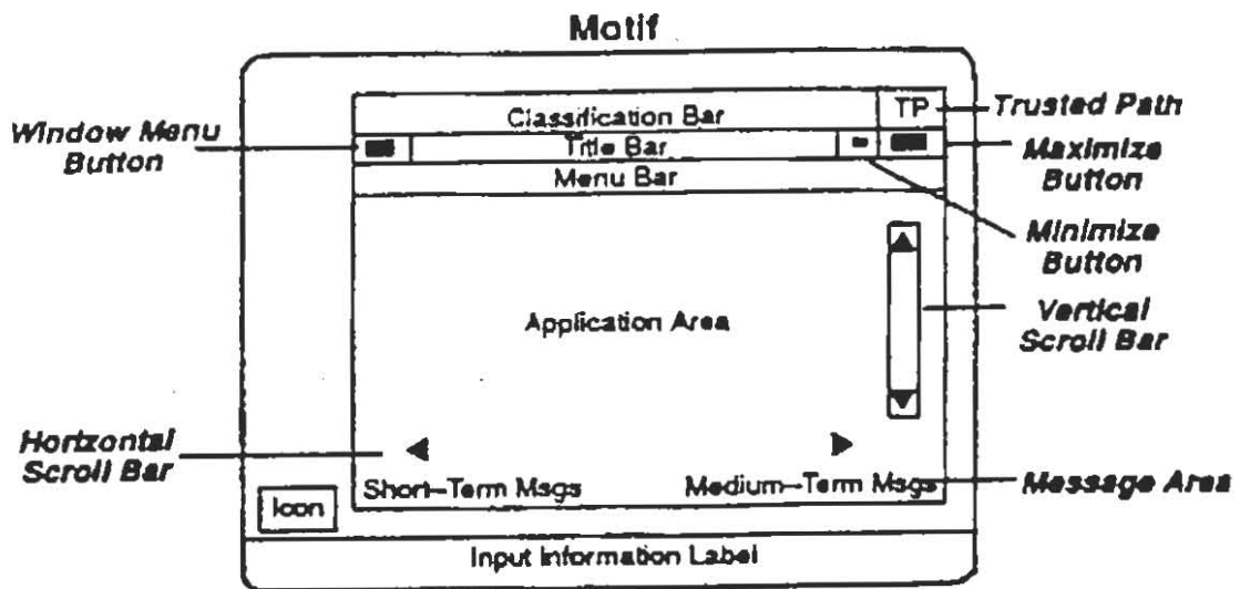
Figure A5-1. Example of a compartmented window.
