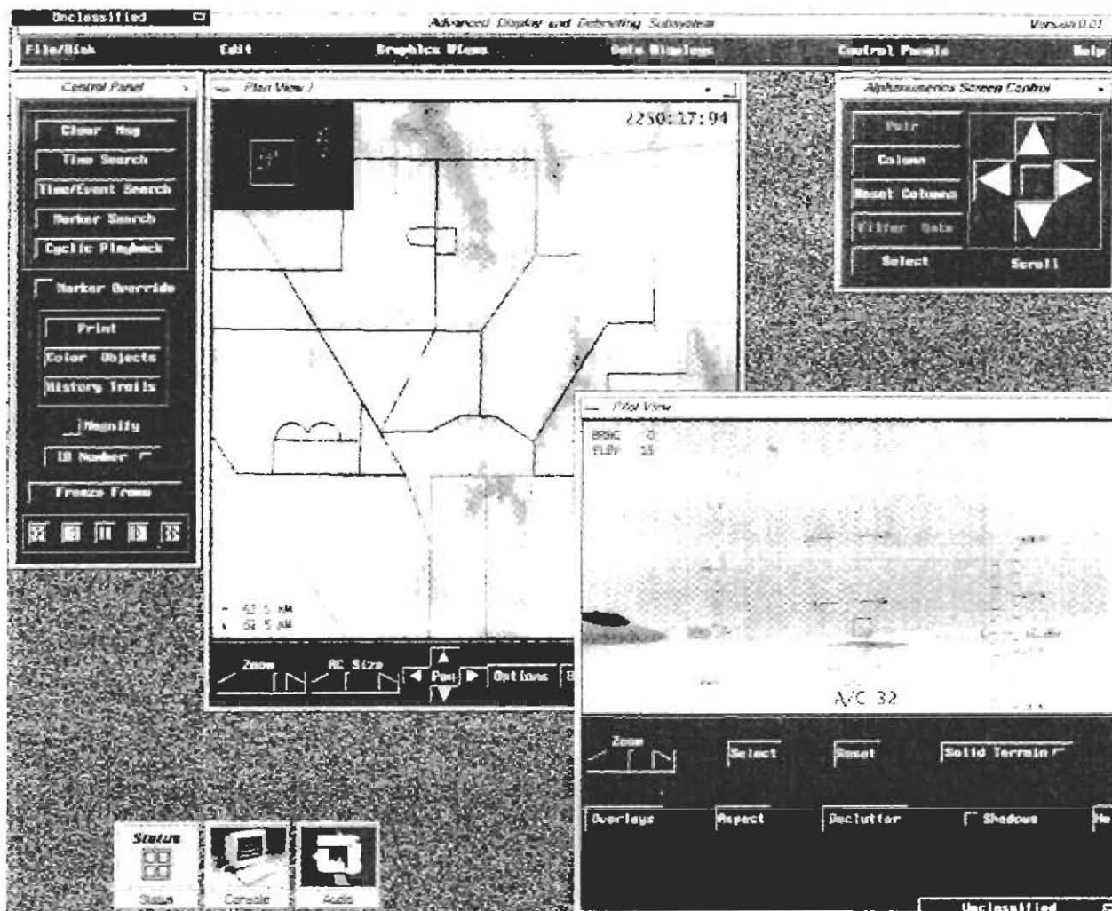
Figure 7-2. Example of Plan View and Pilot View displays.
