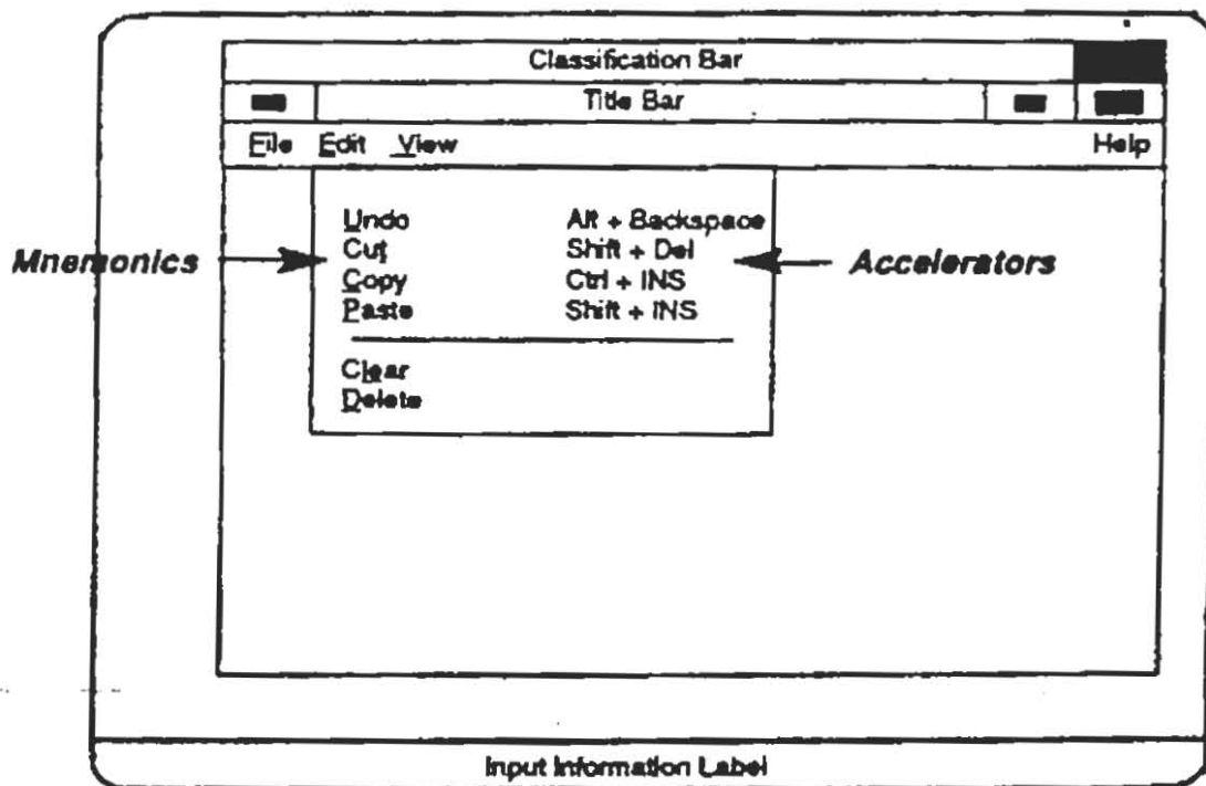
Figure A5-6. Example of the use of mnemonics and accelerators.
