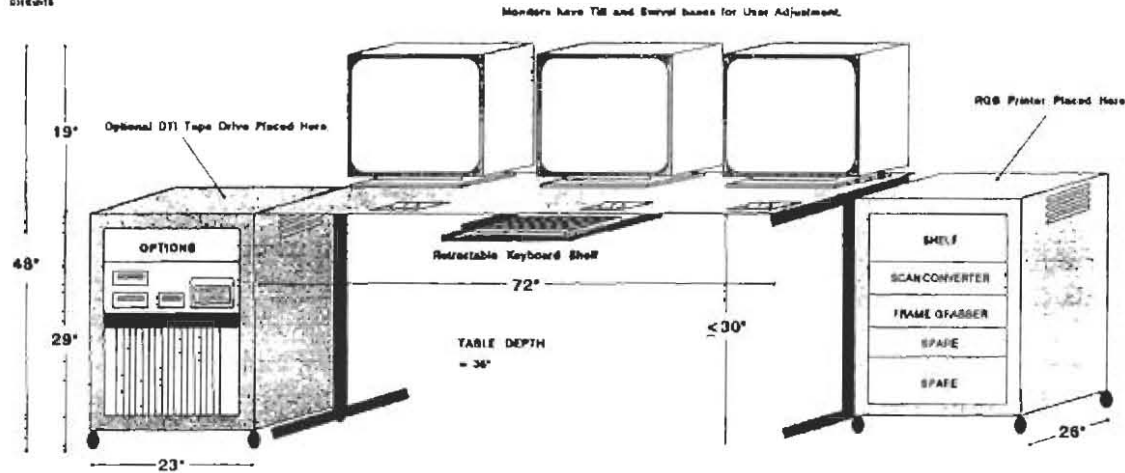
Figure 8-1 Illustration of the basic Type B configuration.
