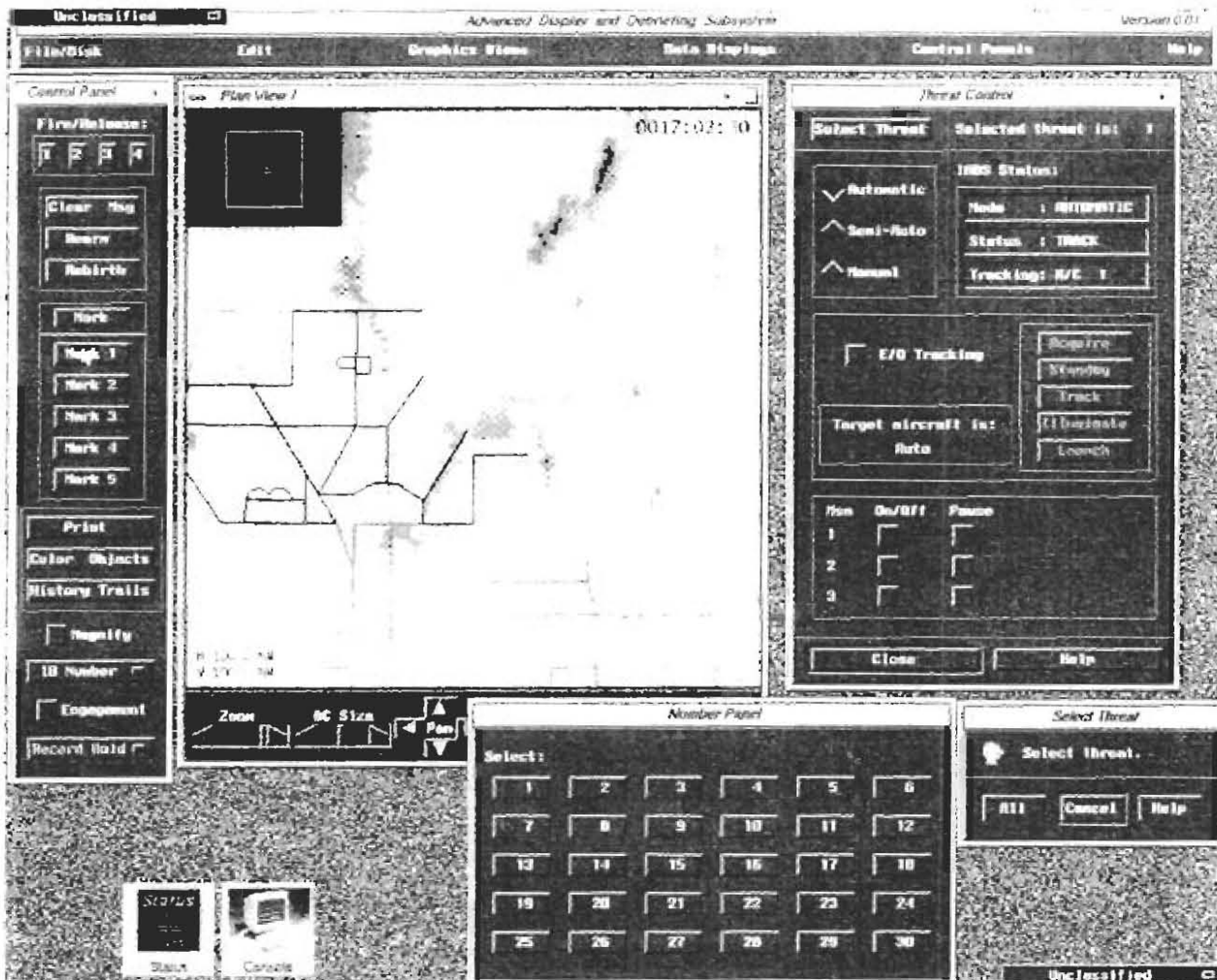
Figure 7-24. Illustration of a good default arrangement for controls panels.
